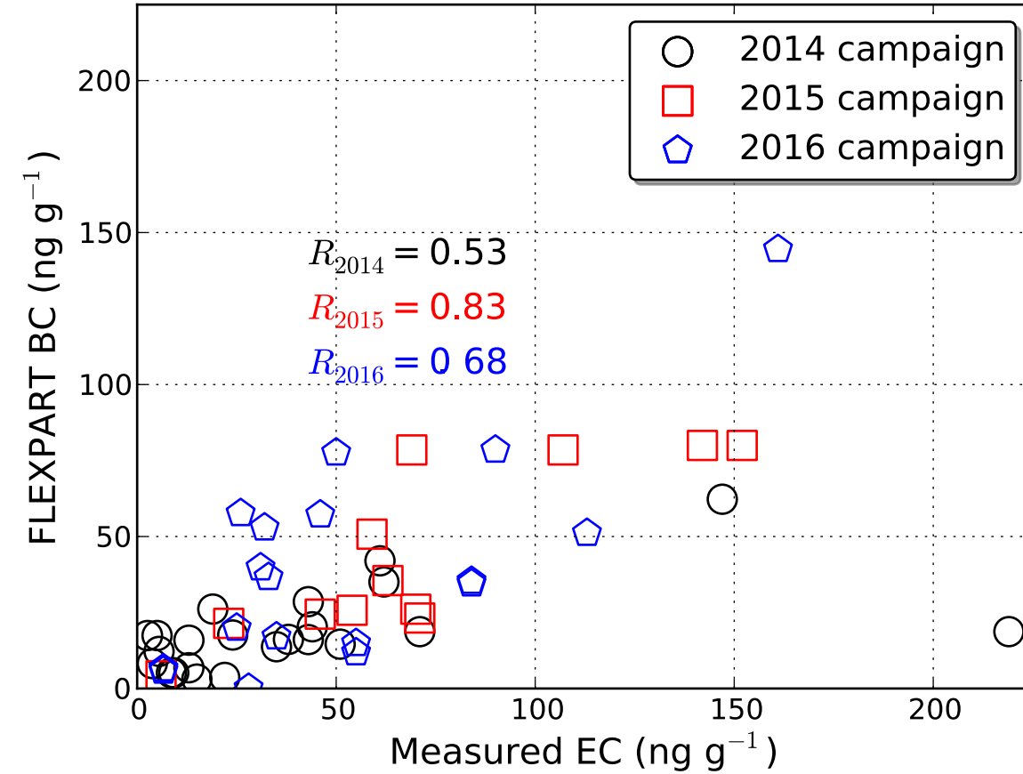
(b) Modelled BC vs. measured EC in snow
