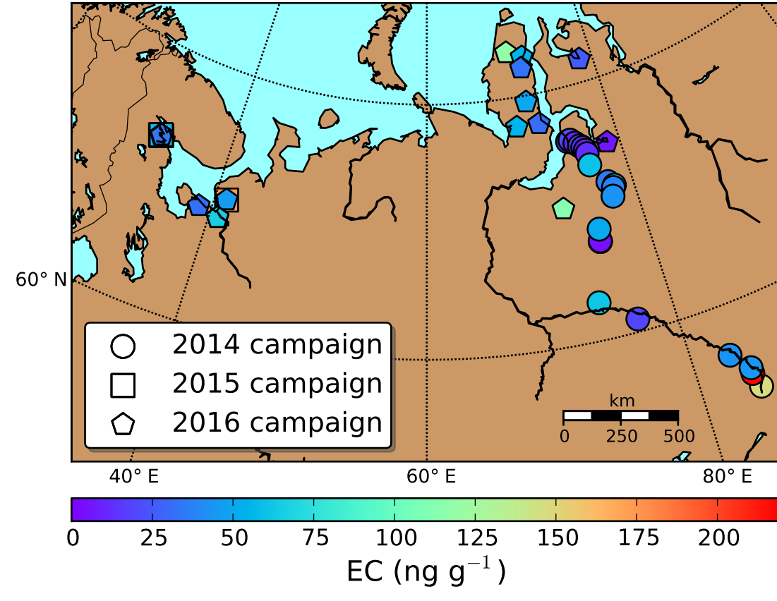
(c) Spatial distribution of EC in snow
