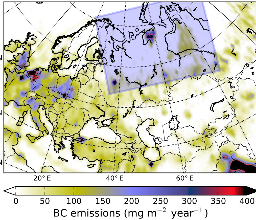
(a) ECLIPSE+GFED4 emissions
