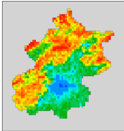
(a) GLASS: JJA
