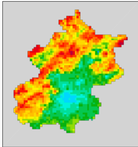
(c) GEO: JJA
