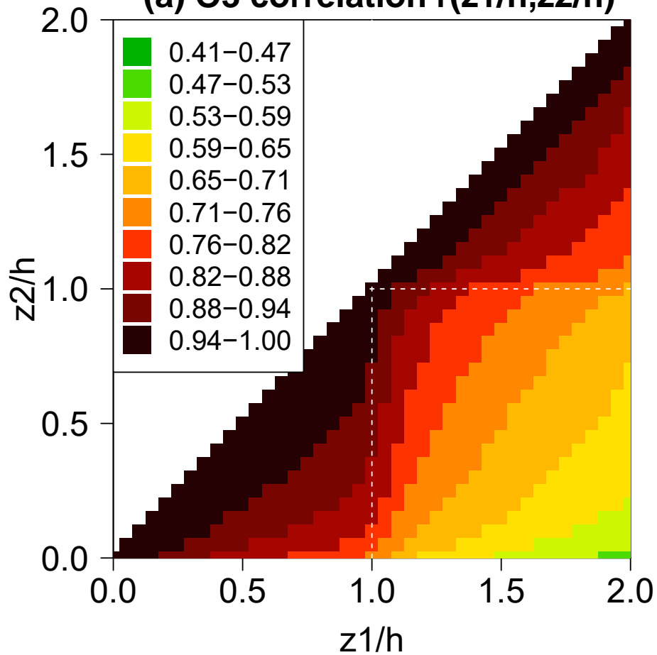
(a) O3 correlation r(z1/h, z2/h)
