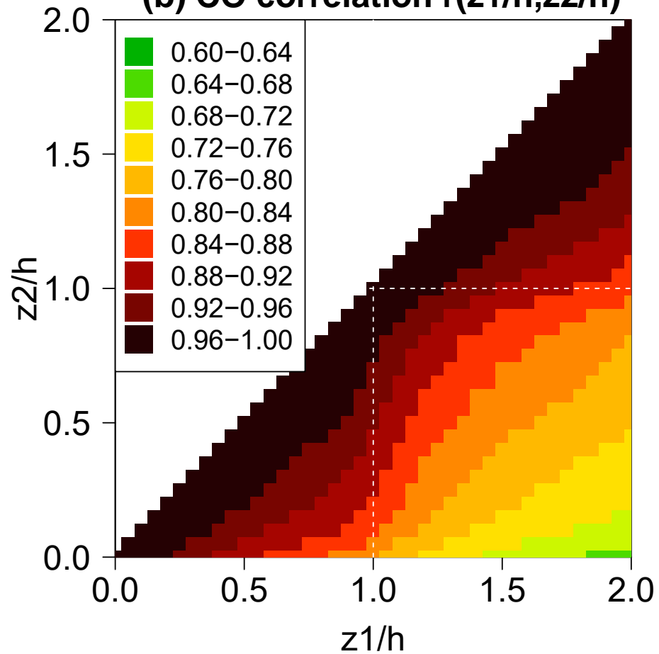
(b) CO correlation r(z1/h, z2/h)
