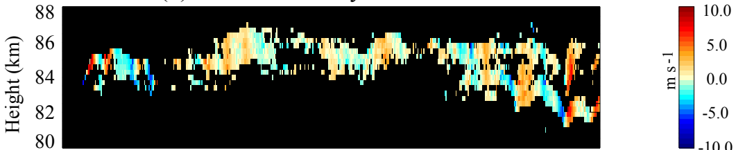
(c) SNR KAIRA
