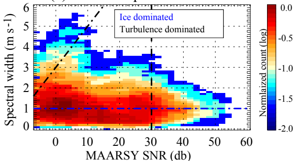
(c) SNR vs. spectral width
