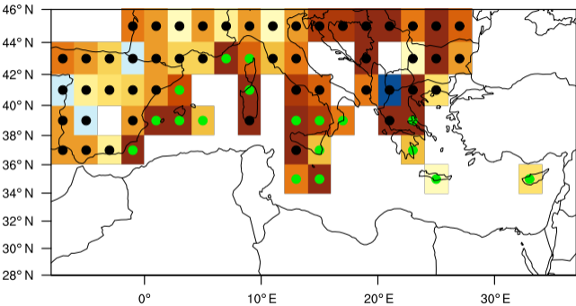
Multimodel mean bias (ppbv)
