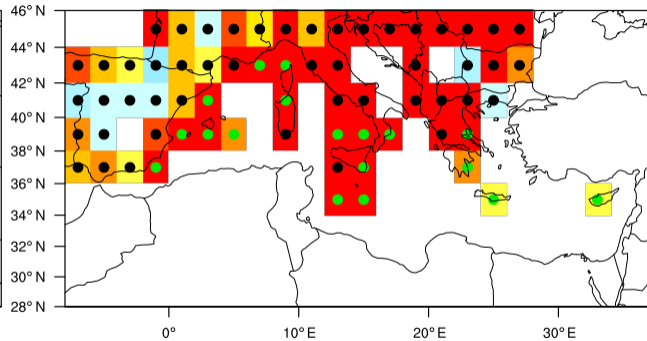
Multimodel mean of absolute error (ppbv)
