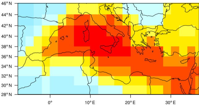
Multimodel mean surface ozone (ppbv)
