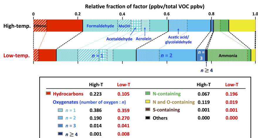
Figure 6. VOC composition in the high- and low-temperature emission profiles.
