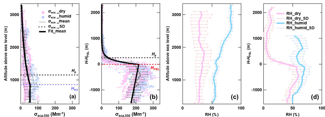
Figure 6. Mean vertical distributions of \sigma_{\text{sca}} at 550 nm (in \text{Mm}^{-1} ) and relative humidity (%) during the flight campaign for those cases of (a, c) clean PBL and (b, d) pollution in the lower layer of the PBL where PBL heights have been normalized to the same altitude. Grey dashed lines represent mean \sigma_{\text{sca}} vertical profiles, the light pink and blue dots represent 1 s nephelometer-measured \sigma_{\text{sca}} , under dry or humid conditions, respectively. Thick lines show the calculated fitting curves of the \sigma_{\text{sca}} profiles (see Eqs. 8 and 9). Magenta and blue lines represent RH data collected under dry or humid conditions (c, d). The horizontal error bars represent the standard deviations at every 100 m level.
