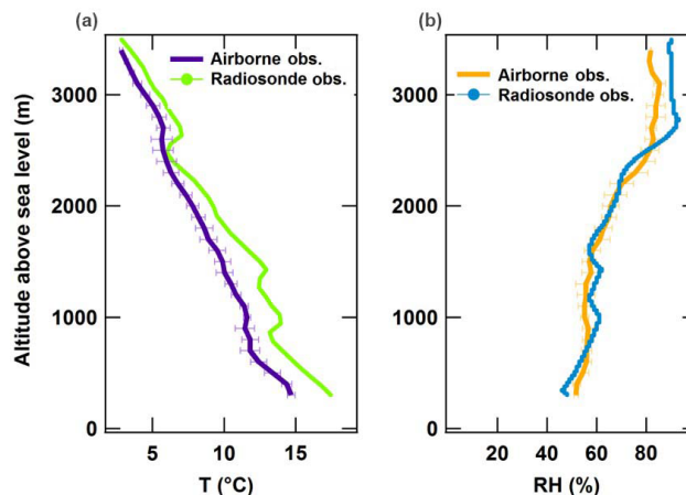
Figure 2. Vertical profiles of temperature ( T , a) and relative humidity (RH, b) from radiosonde and airborne measurements made on 8 May 2016 over the Xingtai supersite. Horizontal bars represented standard deviations.
