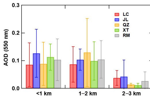
Figure 5. Mean AOD at 550 nm at LC, JL, QZ, and XT, and overall mean AOD (RM) at 550 nm for different altitude ranges (< 1, 1–2, and 2–3 km). Standard deviations are also shown.
