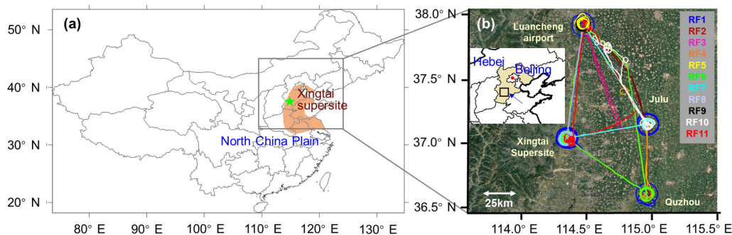
Figure 1. Map of the geographic location of the North China Plain and the Xingtai supersite (a), and the flight tracks of the 11 research flights conducted over Hebei Province during May–June 2016 (b). The orange shaded area denotes the North China Plain.
