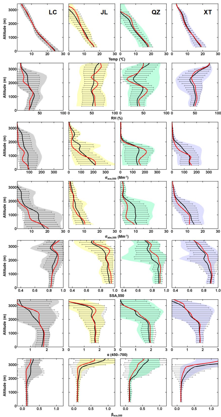
Figure 4. Mean vertical distributions of (from the top row to the bottom row) temperature ( ^{\circ}\text{C} ), relative humidity (%), \sigma_{\text{sca}} at 550 nm ( \text{Mm}^{-1} ), \sigma_{\text{abs}} at 550 nm ( \text{Mm}^{-1} ), SSA at 550 nm, Ångström exponent ( \alpha ), and \beta_{\text{sca}} at 550 nm over LC, JL, QZ, and XT (from the left column to the right column, respectively). Black and red lines represent the mean and the median, respectively, and horizontal bars are standard deviations at every 150 m level. The colored shaded areas represent the 10th and 90th percentiles of the data.
