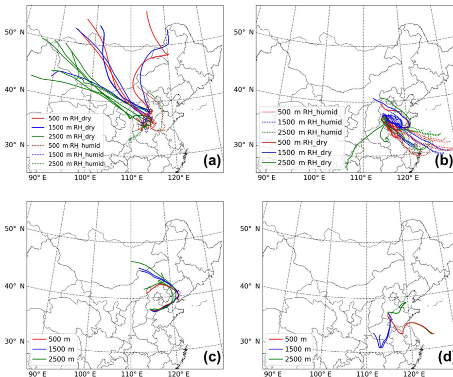
Figure 9. 72 h HYSPLIT back trajectories for the cases when the PBL was (a) clean, (b) polluted in the lower PBL, (c) polluted in the upper PBL in the flight on 2 June, and (d) polluted in multiple layers of the PBL in the flight on 6 June. Trajectories at different levels under dry (solid lines) and humid (dashed lines) conditions are shown: 500 m (red), 1500 m (blue), and 2500 m (green) above mean sea level.
