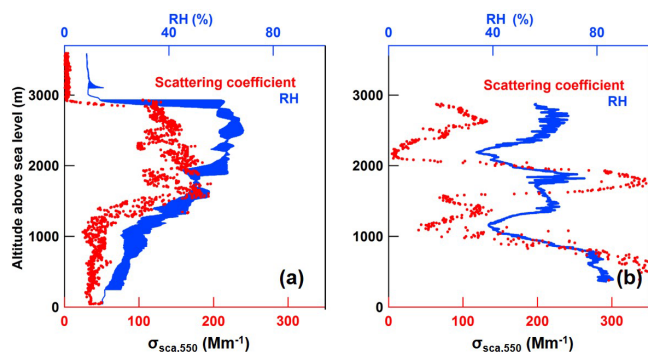
Figure 7. Vertical distributions of \sigma_{\text{sca}} at 550 nm (red) and relative humidity (RH, blue) for the enrichment of aerosols in the upper layer of the PBL on 2 June in LC (a) and in multiple layers of the PBL on 6 June in JL (b).
