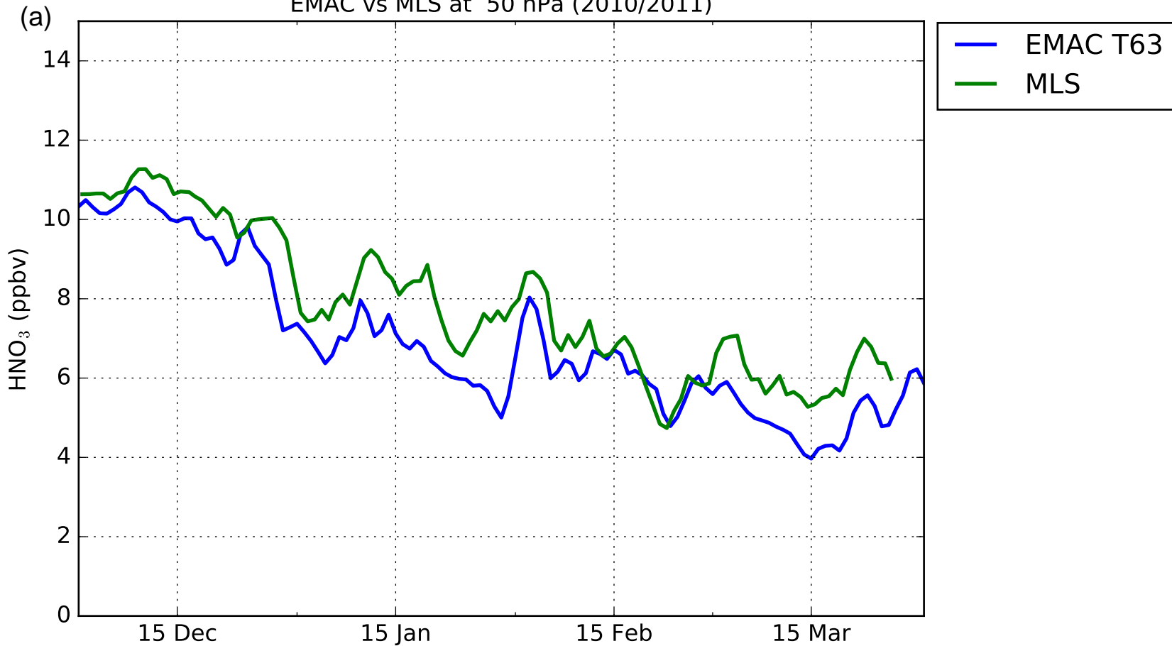
EMAC vs MLS at 50 hPa (2010/2011)
