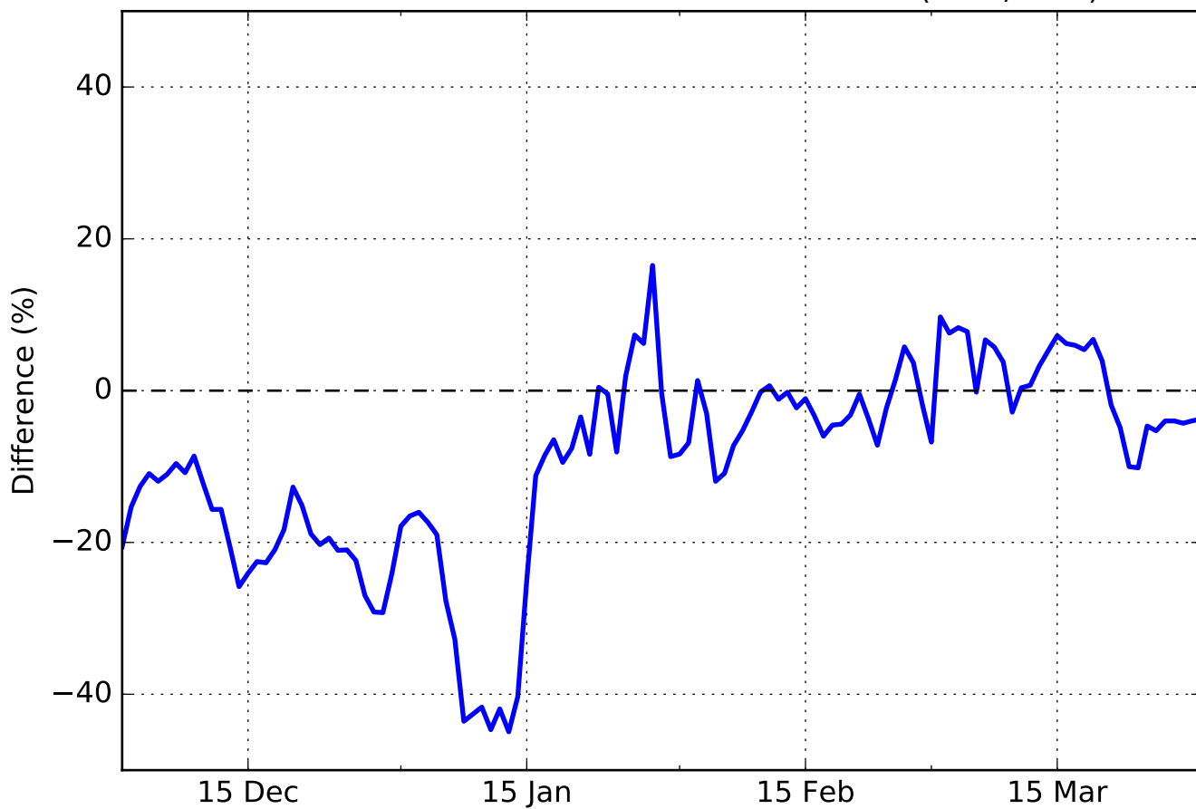
(b) Relative differences EMAC T63 - MLS at 50 hPa (2009/2010)
