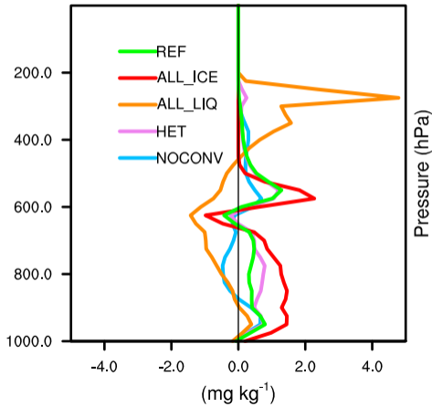
(a) \Delta Cloud water
