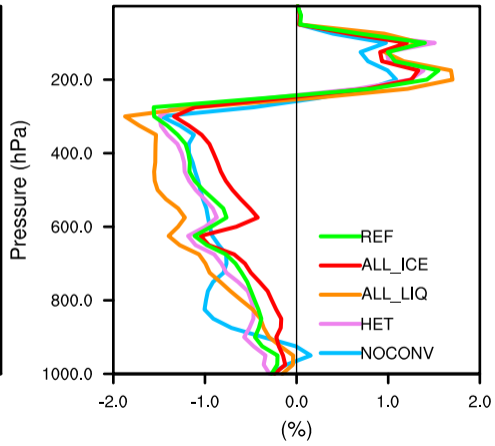
(c) \Delta Cloud fraction
