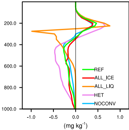
(b) \Delta Cloud ice
