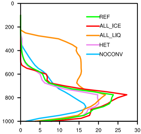
(a) Cloud water ( \text{mg kg}^{-1} )
