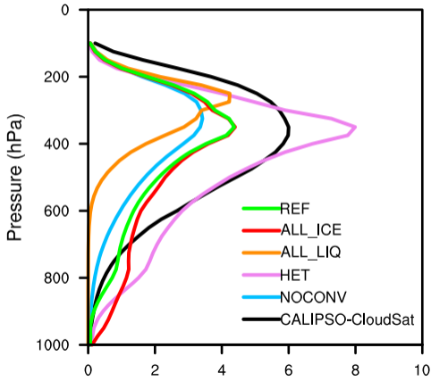
(b) Cloud ice ( \text{mg kg}^{-1} )
