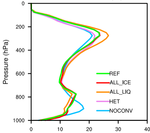
(c) Cloud fraction (%)
