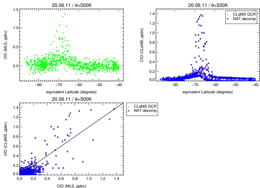
Figure S6. Comparison of MLS ClO observations with CLaMS for 20.06.2011 at 500 K potential temperature pole-ward of 40°S: (a) MLS data vs equivalent latitude, (b) corresponding CLaMS results vs equivalent latitude for runs “GCR” and “NAT decomp”, (c) CLaMS vs MLS.
