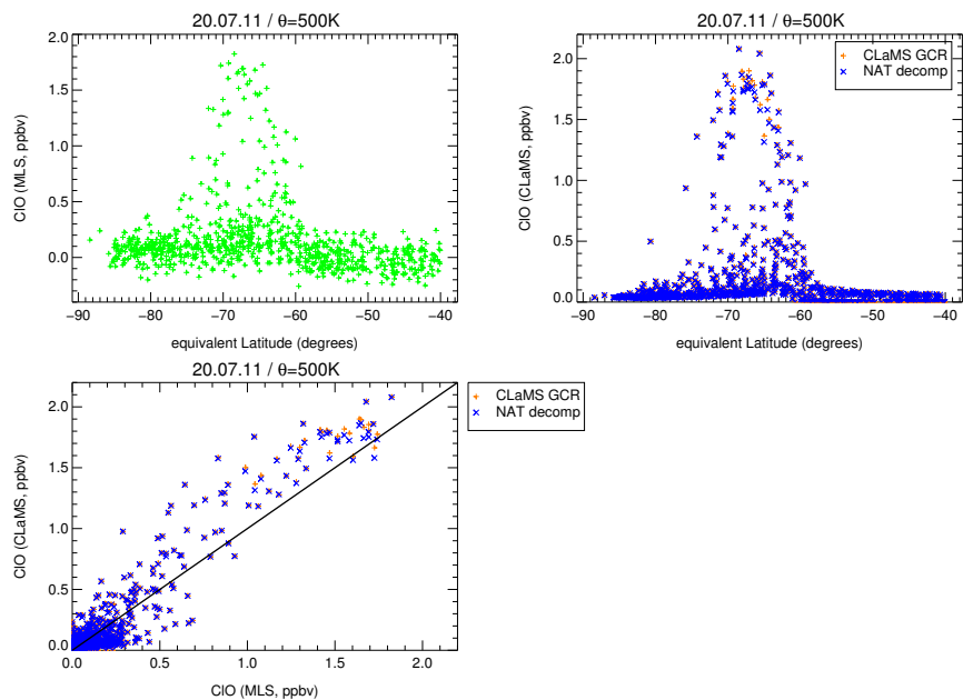
Figure S7. As Figure S6 but for 20.07.2011.
