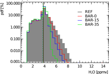
(b) 20° S-20° N / 380-420 K
