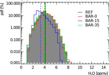
(c) 40° N-90° N / 370-420 K
