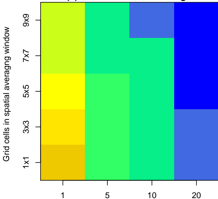
(c) Northeastern US grid cell
