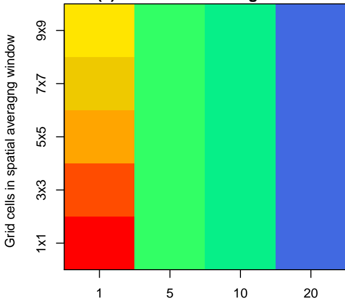
(c) Northeastern US grid cell
