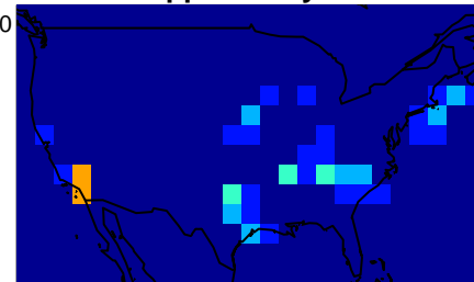
2.5 ppbv / 20-year
