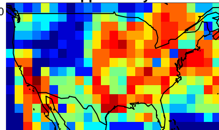
1 ppbv / 10-year
