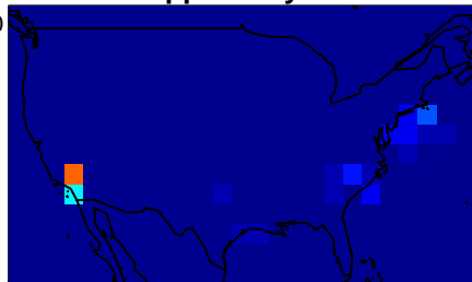
5 ppbv / 5-year
