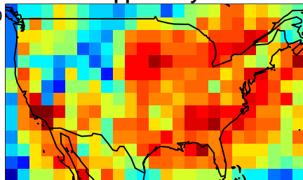
1 ppbv / 5-year
