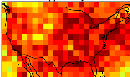
1 ppbv / 1-year
