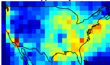
5 ppbv / 1-year
