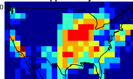
1 ppbv / 20-year
