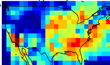
2.5 ppbv / 5-year
