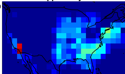
5 ppbv / 5-year
