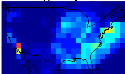
5 ppbv / 1-year
