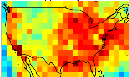
2.5 ppbv / 1-year
