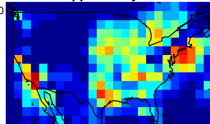
2.5 ppbv / 10-year
