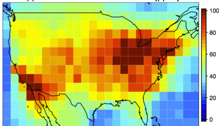
(f) Future 2100 CAM-Chem mean [ppbv]
