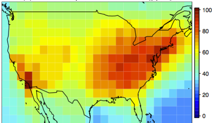
(c) Present-day CAM-Chem SD [ppbv]
