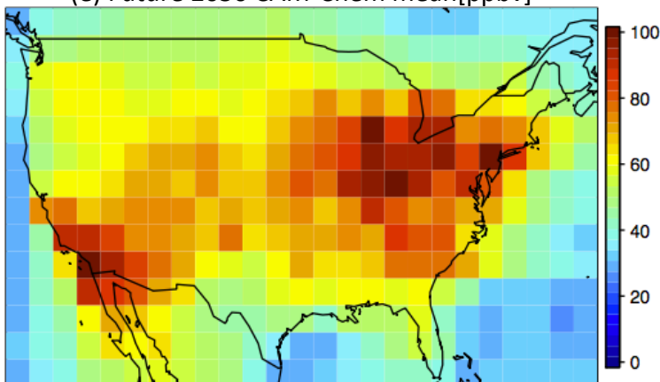
(e) Future 2050 CAM-Chem mean [ppbv]
