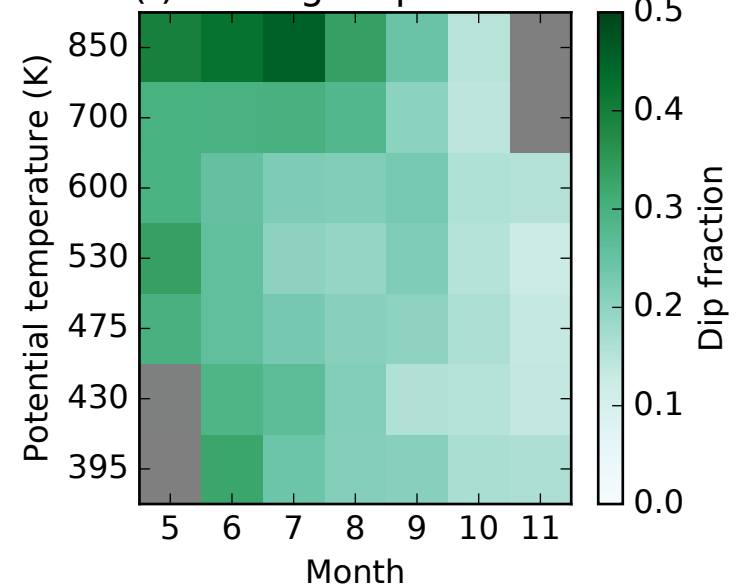
(f) Average dip fraction
