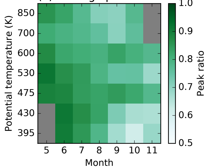
(e) Average peak ratio
