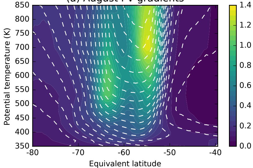
(a) August PV gradients
