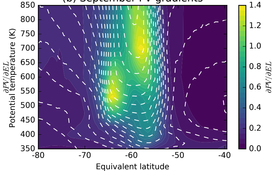
(b) September PV gradients
