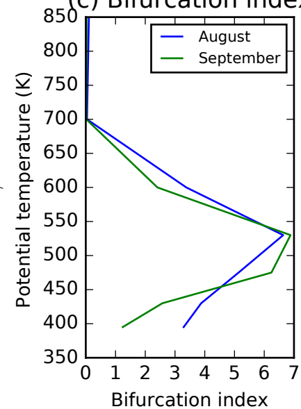
(c) Bifurcation index
