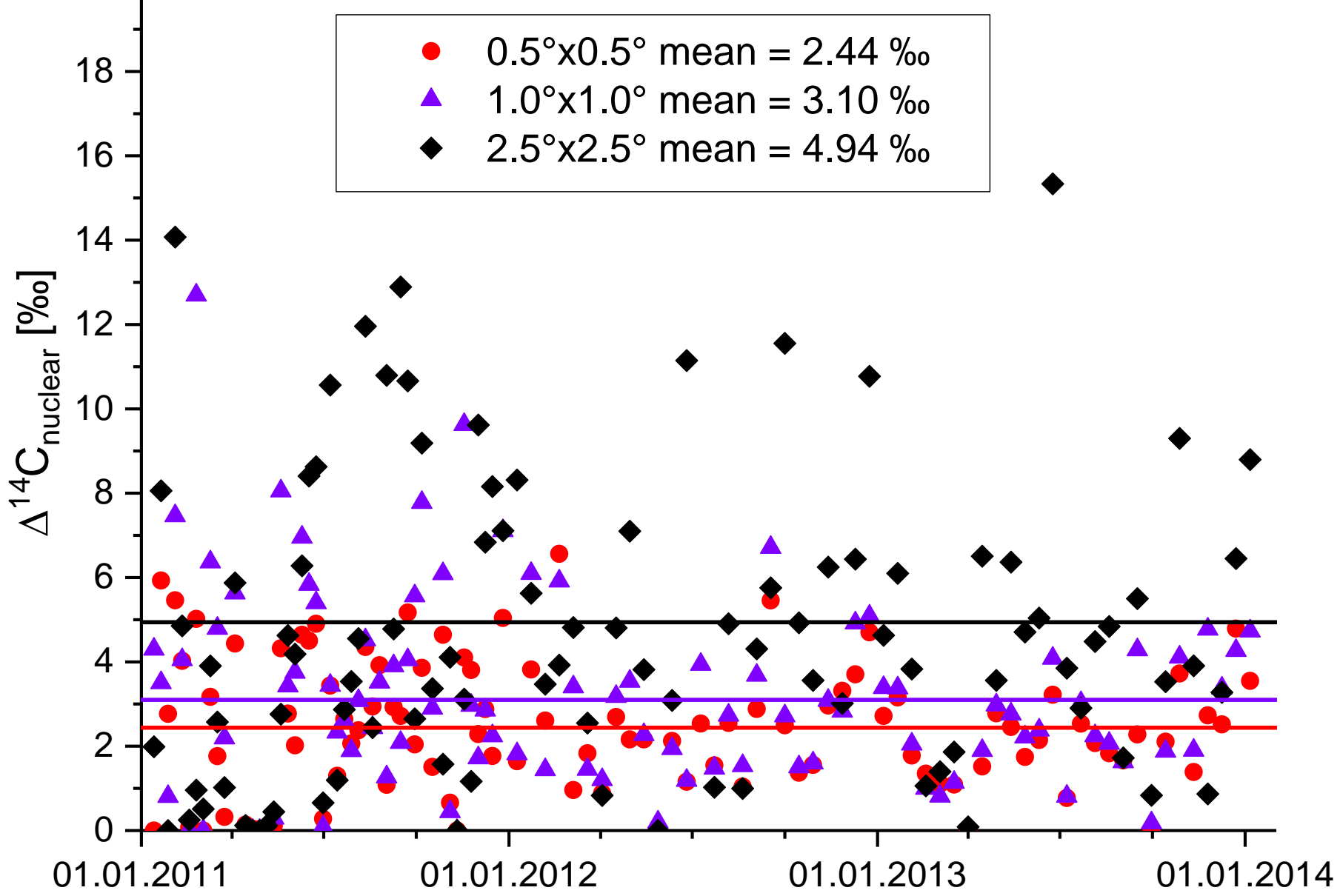
(a) Philippsburg (KKP I & II) with 0.45 TBq ^{14}\text{CO}_2 \text{ yr}^{-1}
