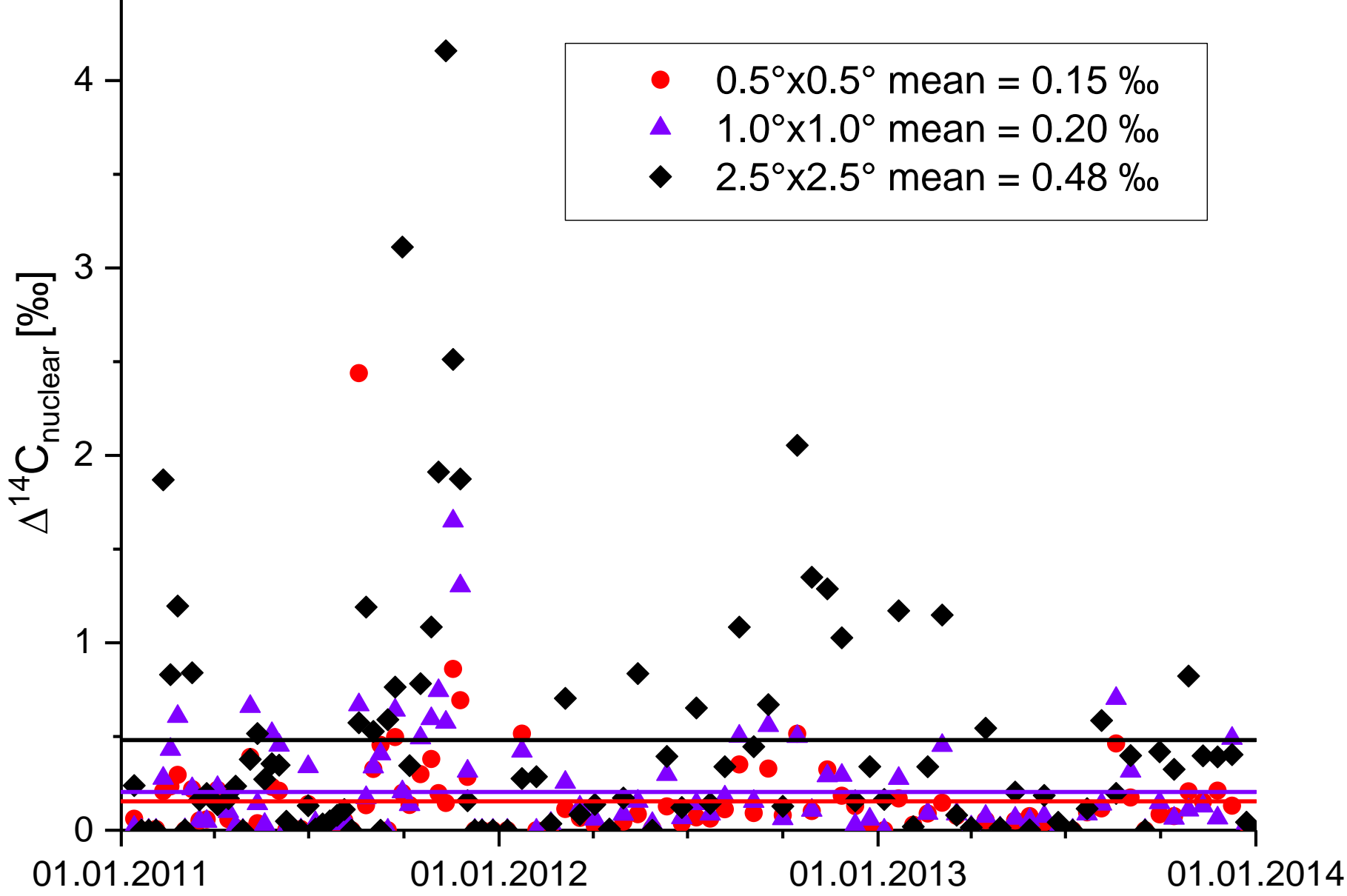
(b) Neckarwestheim (GKN I & II) with 0.12 TBq ^{14}\text{CO}_2 \text{ yr}^{-1}
