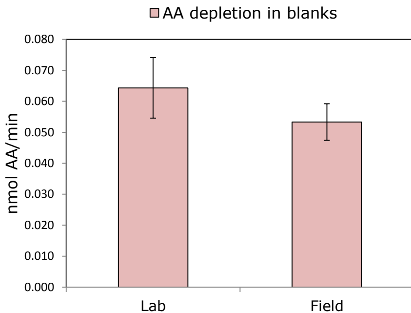
Figure S3 : AA depletion in laboratory (n=7) and field (n=6) blank filters analyzed in triplicates.
