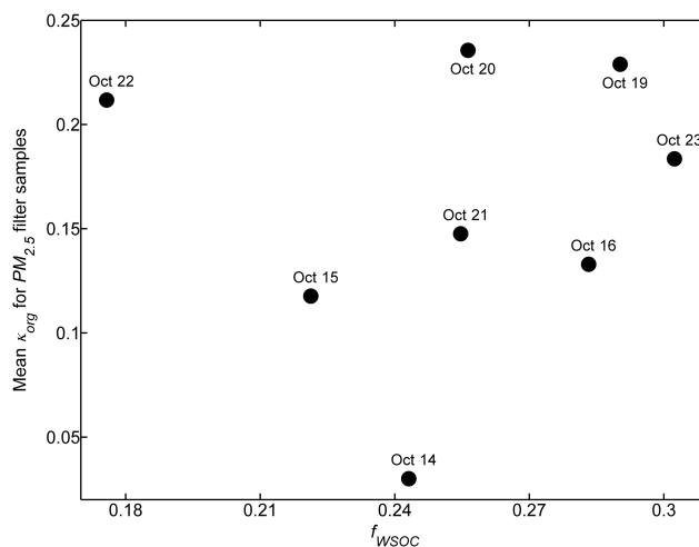
Figure 8. Correlation between the mean \kappa of organics ( \kappa_{\text{org}} , with 10.0 % EC mass fraction considered in the \kappa calculation) and the mean WSOC fraction ( f_{\text{WSOC}} ) of \text{PM}_{2.5} filter samples.
