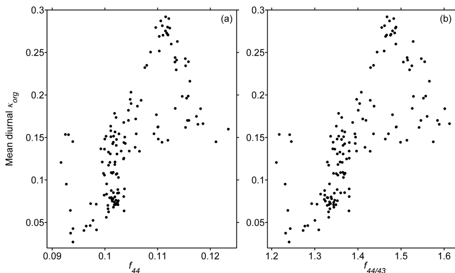
Figure 9. Relationships between the mean diurnal \kappa_{\text{org}} results vs. (a) f_{44} and (b) f_{44/43} in NR-PM 1 haze particles. Mean diurnal here represents that the diurnal results for each day were further averaged over the overlapping observation period, i.e., with both HTDMA and ToF-ACSM measurements taken from 10 to 24 October 2015.
