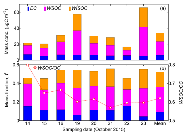
Figure 4. (a) Mass concentration (“Mass conc.”, \mu\text{gC m}^{-3} ) and (b) corresponding mass fraction, f , of the carbon contents including EC, WSOC, and water-insoluble OC (WISOC) in \text{PM}_{2.5} filter samples. The WSOC / OC ratio is also displayed by the scattered dots in (b). All the corresponding temporal mean results are shown as “Mean”. The WSOC fraction was exclusively higher than that of WISOC or EC, highlighting the dominance of WSOC in the carbon content of \text{PM}_{2.5} filter samples. In general, the EC fraction fluctuated around 10.0 % of the total \text{PM}_{2.5} mass.
