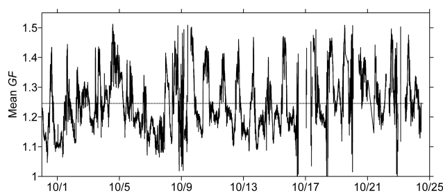
Figure 5. Time series of the volume-weighted mean particle diameter growth factor (GF) derived from HTDMA measurements (date format: month/day, 2015). The black dashed line stands for the temporal mean GF averaged over the entire observation period.
