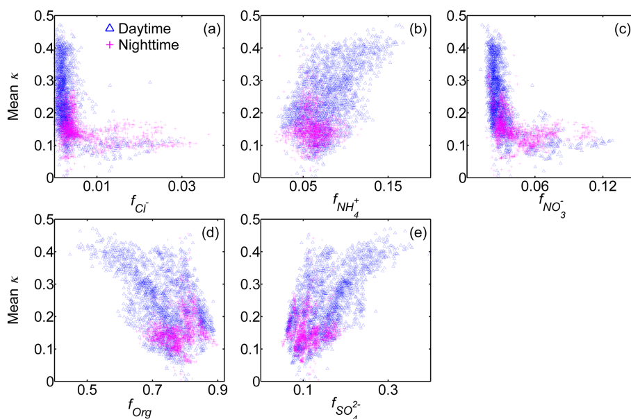
Figure 7. Relationships between the mean \kappa results (100 nm) and the mass fractions of the five non-refractory chemical compositions of submicron wildfire haze particles.
