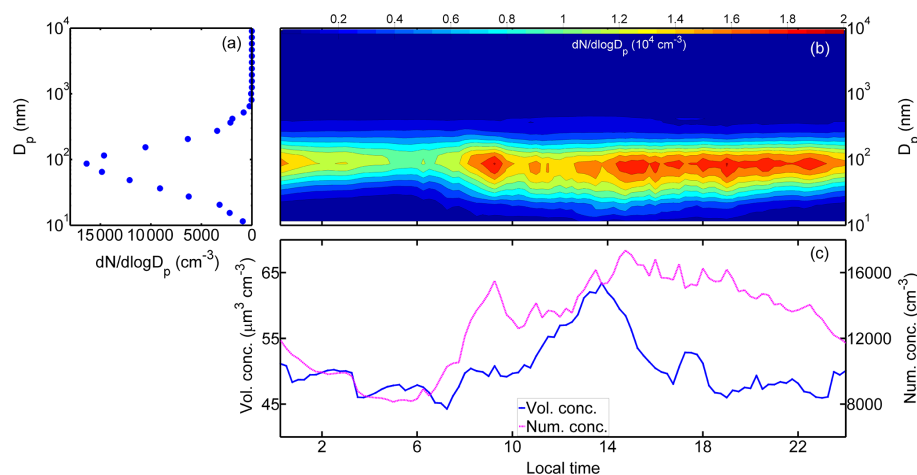
Figure 2. (a) The mean particle number size distribution ( dN/d\log D_p , \text{cm}^{-3} ) during the ambient wildfire haze observations as well as the mean diurnal variations of (b) particle size distribution, (c) number concentration (“Num. conc.,” \text{cm}^{-3} , denoted by the magenta solid line), and volume concentration (“Vol. conc.,” \mu\text{m}^3 \text{cm}^{-3} , as the blue line displayed) measured with NanoScan-SMPS (11.5–365.2 nm) and OPS (419 nm–10 \mu\text{m} ) (local time, LT). High aerosol loading was commonly observed during the transboundary wildfire haze. Submicron particles in the size range of 30–200 nm dominated the total number concentration of wildfire haze particles.
