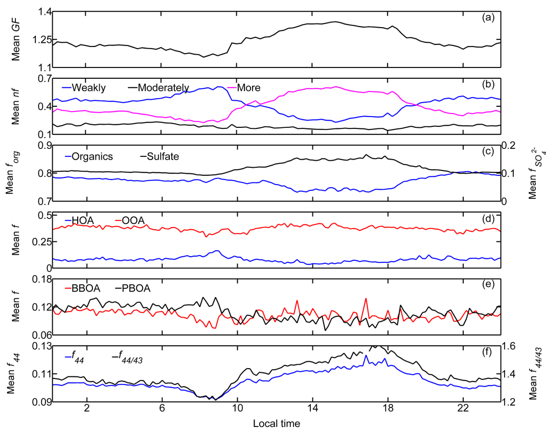
Figure 6. Temporally averaged (10–24 October 2015) diurnal variations of (a) the mean GF; (b) number fraction (nf) of the three hygroscopic modes; (c) mass fraction of the two main components in NR-PM 1 , i.e., organics ( f_{\text{org}} ) and sulfate ( f_{\text{SO}_4^{2-}} ); (d, e) mass fraction of the ME-2-resolved four OA factors in NR-PM 1 (i.e., f_{\text{HOA}} , f_{\text{OOA}} , f_{\text{BBOA}} , and f_{\text{PBOA}} ); and (f) mean f_{44} and f_{44/43} of organics in NR-PM 1 (local time, LT). Pronounced diurnal patterns were observed for the mean GF, number fractions of both weakly and more hygroscopic modes, f_{44} , f_{44/43} , and mass fractions of organics and sulfate as well as HOA and OOA; \text{nf}_{\text{more}} , f_{\text{SO}_4^{2-}} , f_{44} , f_{44/43} , and f_{\text{OOA}} showed variations similar to that of the mean GF, whereas contrasting diurnal patterns were found for \text{nf}_{\text{weakly}} , f_{\text{org}} , and f_{\text{HOA}} .
