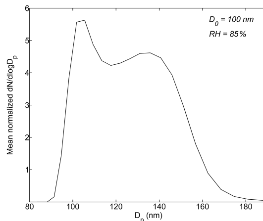
Figure 1. Normalized particle number size distribution ((dN/d\log D_p)/N) after humidification averaged over the entire haze observation period.
