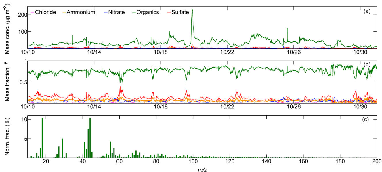
Figure 3. Time series of (a) mass concentration (“Mass conc.”, \mu\text{g m}^{-3} ) and (b) corresponding mass fraction, f , of the five specific chemical species in NR-PM 1 measured by ToF-ACSM (abscissa shows the observation dates in October 2015 in the date format of month day -1 ). (c) Temporally averaged OA mass spectra for submicron wildfire haze particles, displayed with the normalized ion fraction (Norm. frac., %) of each ion fragment. Wildfire haze particles were predominantly composed of organics. Ion signals ( m/z ) from oxygenated organics (e.g., m/z 43, 44) were prominent, while intensities of ions for hydrocarbon-like organic compounds (e.g., m/z 41, 55, 57) and biomass burning tracers (e.g., m/z 60, 73) were relatively less intense. See the text for details.
