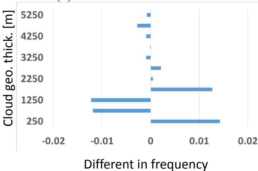
(a) \text{MaxZe} < -15 \text{ dBZ}
