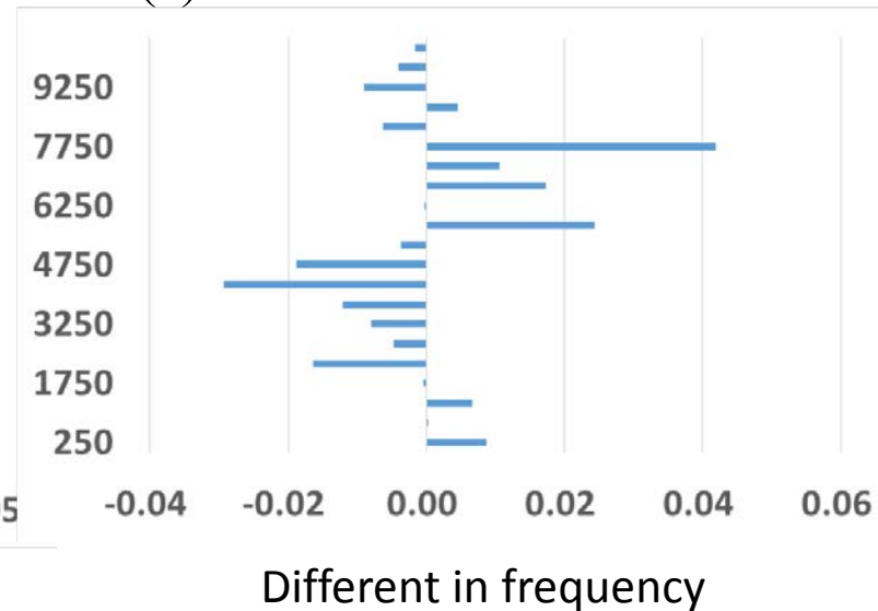
(c) 0 \text{ dBZ} < \text{MaxZe}
