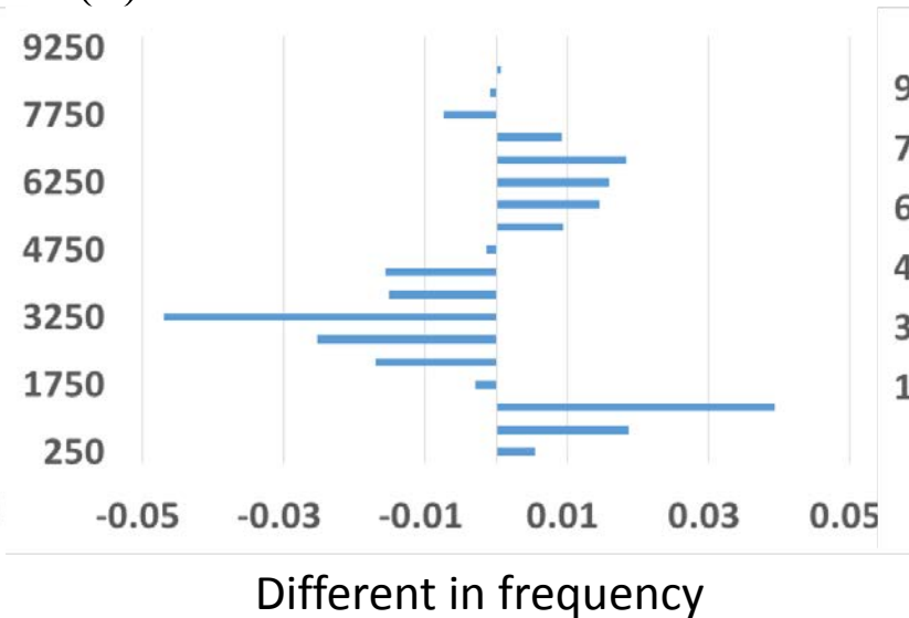
(b) -15 \text{ dBZ} < \text{MaxZe} < 0 \text{ dBZ}
