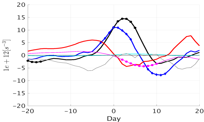
(b) Enstrophy budget, WQBO
