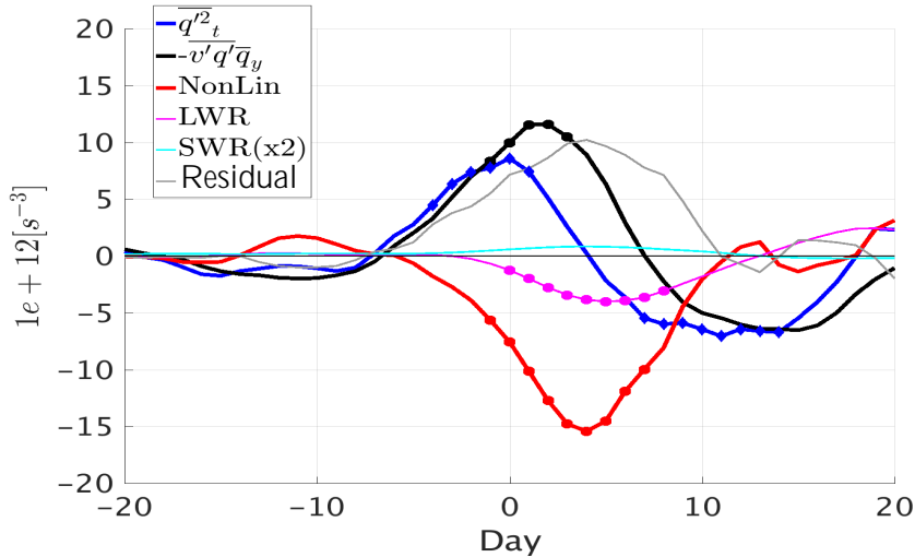
(a) Enstrophy budget, EQBO
