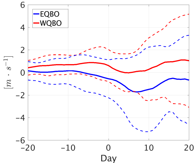
(b) \overline{U} ( \frac{m}{s} ), 50–0.1 hPa, 85–40° N
