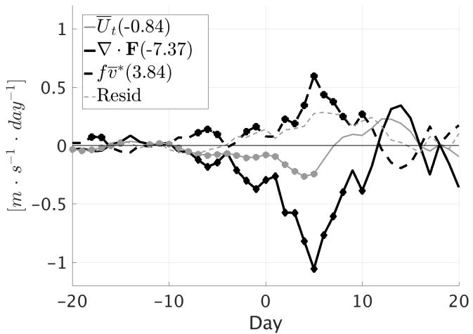
(c) Momentum budget ( \frac{m}{s \cdot day} ), 50–0.1 hPa, EQBO
