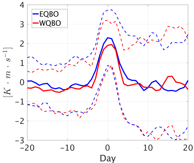
(a) \overline{V'T} ( \frac{m \cdot K}{s} ), 100 hPa, 85–45° N
