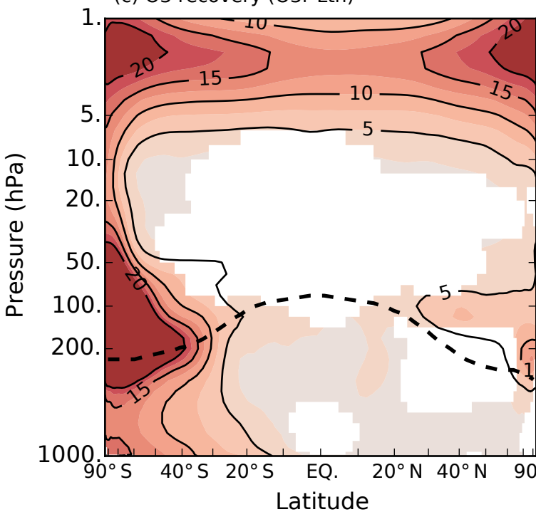
(c) O3 recovery (O3r-Ltn)
