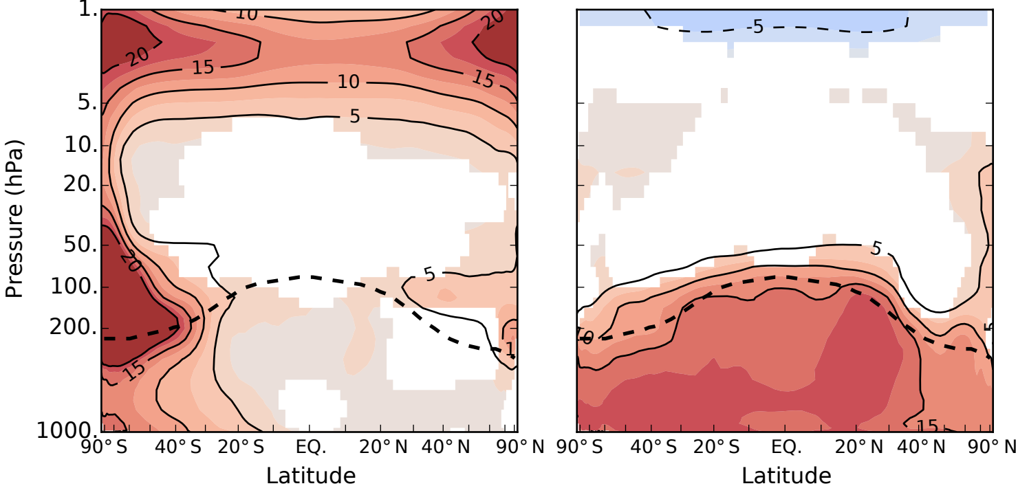
(c) O3 recovery (O3r-Ltn)
