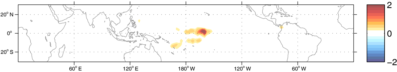
(c) Cloud ice anomaly, 85 hPa, December 2015 [ppmv]
