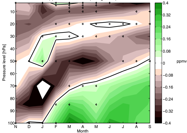
(c) El Nino 2015/2016 (5 integrations)
