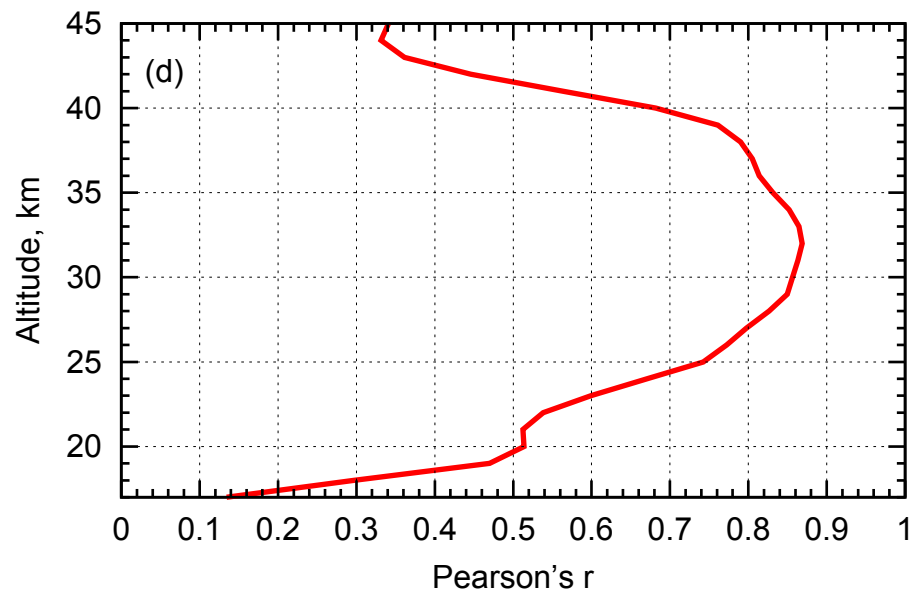
Correlation coefficient SCIAMACHY - ACE profiles
