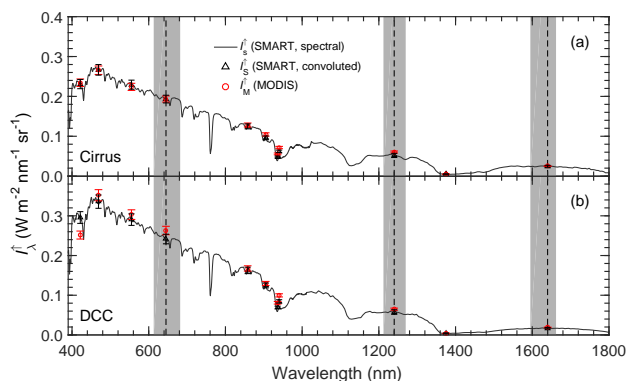
Figure 7. Comparison of mean I_{\lambda}^{\uparrow} measured by SMART and MODIS for the cirrus case (a) and the DCC case (b) at \lambda between 400 and 1800 nm. Error bars represent measurement uncertainties. Wavelengths centered at \lambda = 645 , 1240, and 1640 nm are indicated by dashed lines, while grey bands correspond to the interval of MODIS relative spectral response R(\lambda) for the respective wavelengths.
