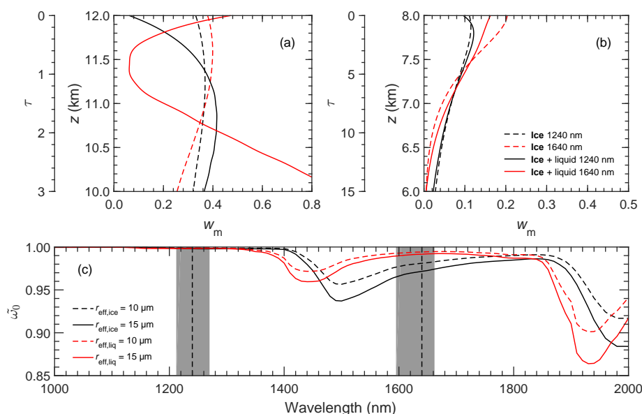
Figure 12. (a) The w_m calculated for cloud A at \lambda = 1240 and 1640 nm, while panel (b) is for cloud B. Solid line and dashed line describe w_m calculated with and without the presence of underlying liquid water cloud, respectively. (c) Single scattering albedo \omega_0 of GHM and liquid water droplets with r_{\text{eff}} of 10 and 15 \mu\text{m} .
