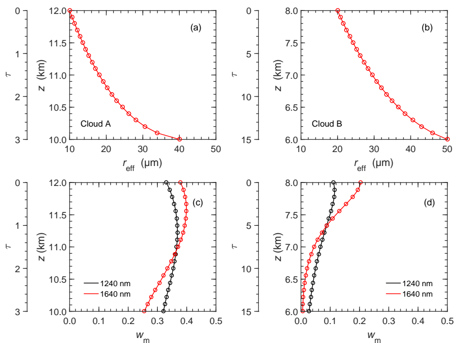
Figure 10. Panel (a) shows an analytic r_{\text{eff}} profile of a cirrus (cloud A) while (b) is for a DCC composed of ice particles only (cloud B). Detailed specifications of the two analytic profiles are summarized in Table 3. Panel (c) is the w_m calculated for cloud A at \lambda = 1240 and 1640 nm, while (d) is for cloud B.
