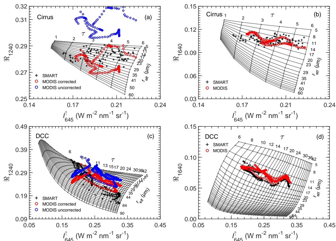
Figure 8. Radiance lookup tables for the cirrus case (a, b) and DCC case (c, d). Panels (a) and (c) are using C1 ( I_{645}^{\uparrow} and R_{1240} ), while (b) and (d) are using C2 ( I_{645}^{\uparrow} and R_{1640} ). For the cirrus case, the simulations are performed with \theta_0 = 37^\circ and assuming GHM (Baum et al., 2014), while for the DCC case \theta_0 = 26^\circ and the ice habit of plate (Yang et al., 2013) are applied. Radiance measurements of SMART and MODIS are illustrated by symbols.
