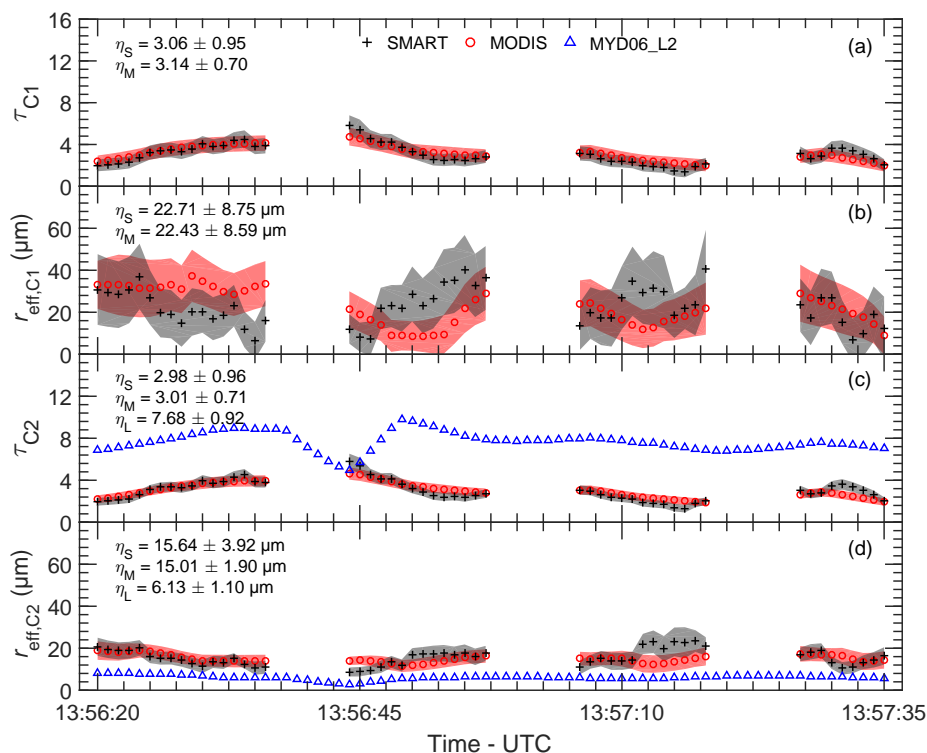
Figure 13. Time series of cirrus \tau (a) and r_{eff} (b) retrieved from SMART (black) and MODIS (red) using combination 1 (C1). The dark shaded area describes retrieval uncertainties. \eta_S (SMART) and \eta_M (MODIS) represent the mean standard deviation along time series. Panels (c) and (d) are the respective properties retrieved using combination 2 (C2). Cloud properties derived from the MODIS cloud product (MYD06_L2), \tau_L and r_{eff,L,2130} , are shown in blue (only in panels c and d) with the corresponding \eta_L .
