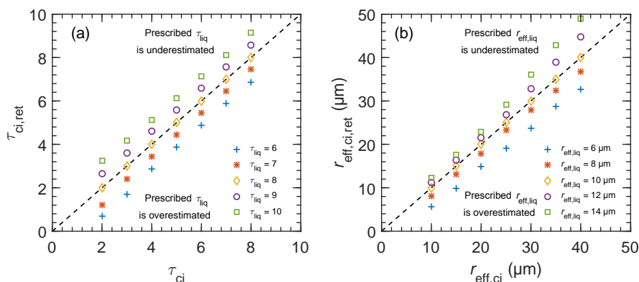
Figure 9. Comparison of synthetically retrieved \tau_{ci} (a) and r_{eff,ci} (b). Calculations in panel (a) are performed by changing \tau_{liq} , while the original value is 8. r_{eff,ci} = 20 \mu\text{m} and r_{eff,liq} = 10 \mu\text{m} are fixed. In panel (b), r_{eff,liq} is changed, while the original value is 10 \mu\text{m} . \tau_{ci} = 3 and \tau_{liq} = 8 are fixed.
