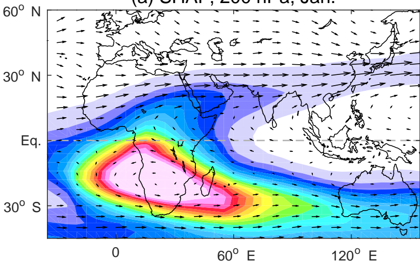
(a) SHAF, 200 hPa, Jan.
