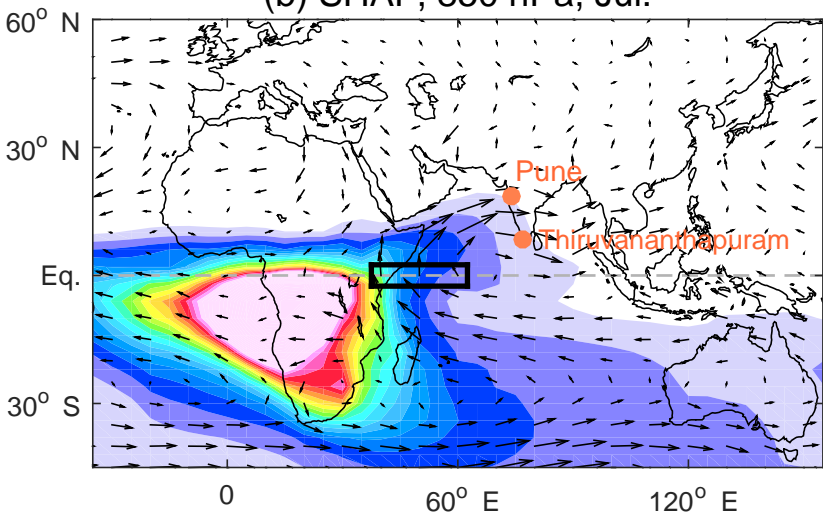
(b) SHAF, 850 hPa, Jul.
