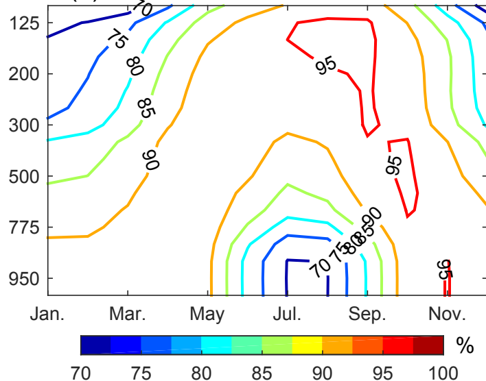
(b) Fractional contribution of NHAF
