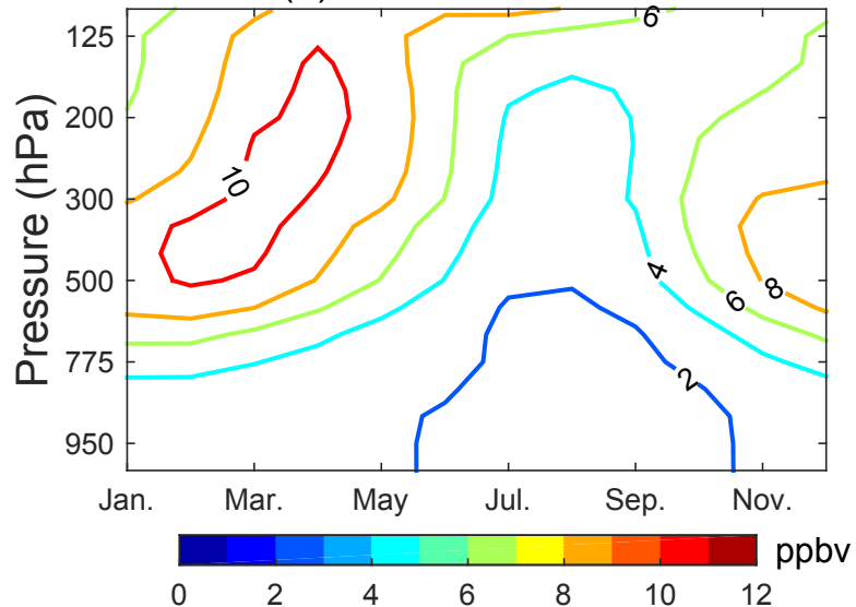
(a) Ozone from NHAF
