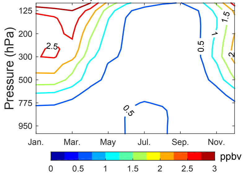
(c) Ozone from SHAF
