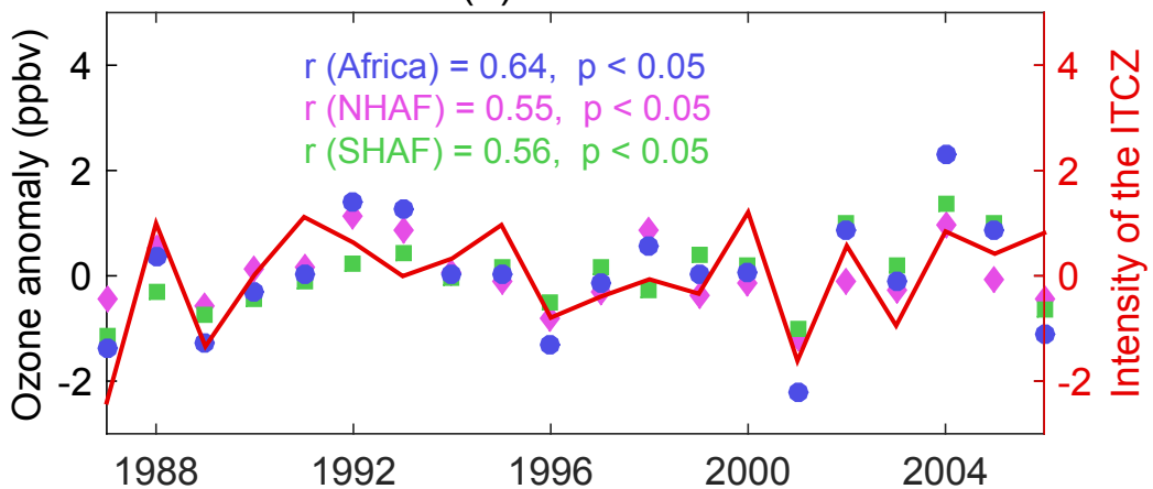
(a) 200 hPa
