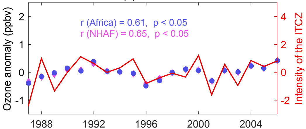
(c) 975 hPa
