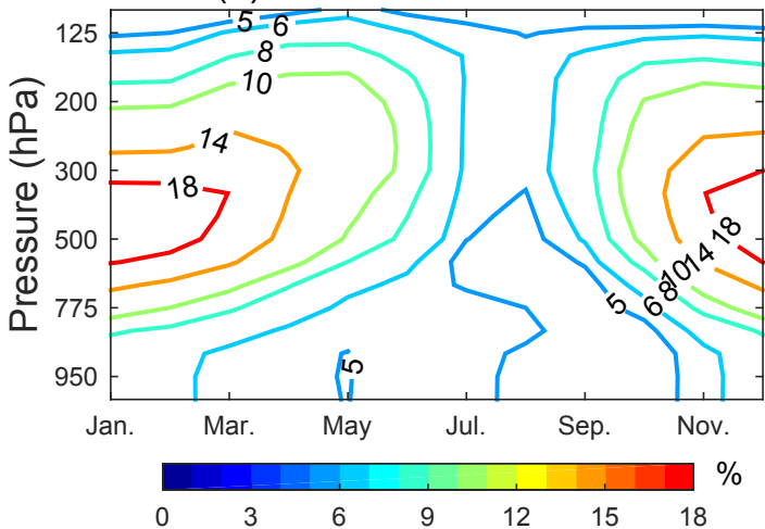
(b) Fractional contribution
