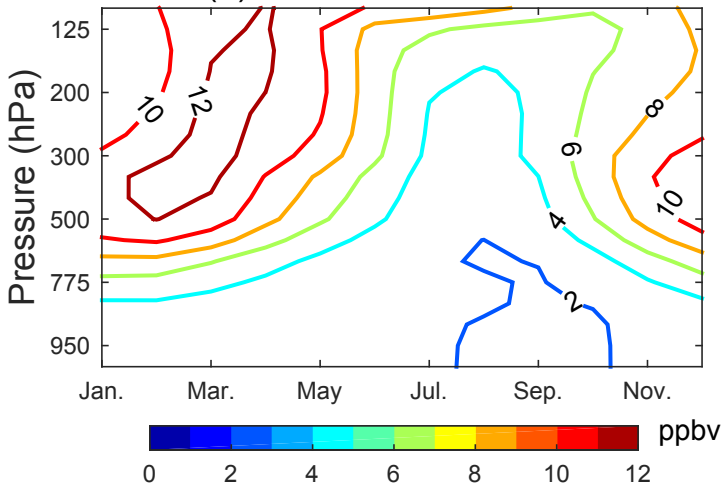
(a) African ozone in Asia
