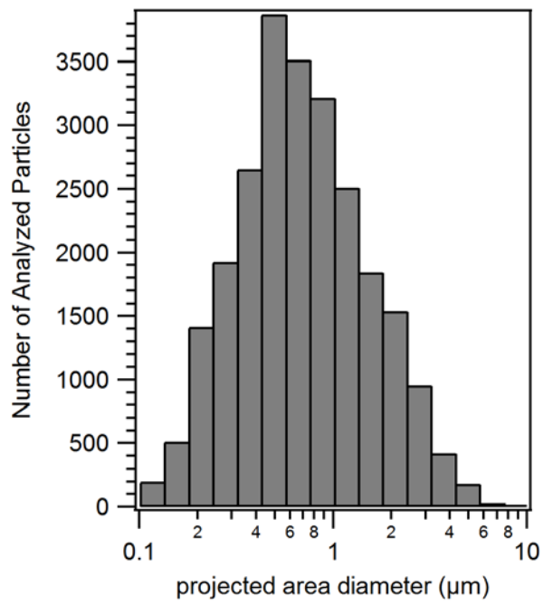
20 Figure S1: The number of individual particles analyzed by CCSEM-EDX for each of 16 log size 21 bins.
