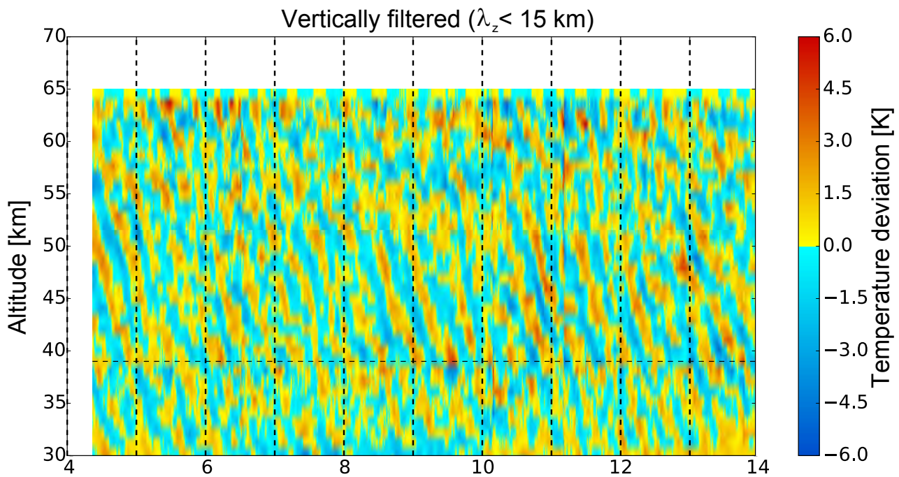
(a) Temperature deviations induced by GW
