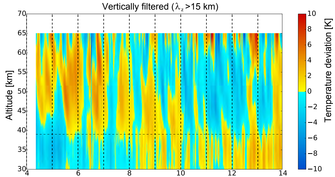
(b) Induced by large scale waves (e.g. tides)
