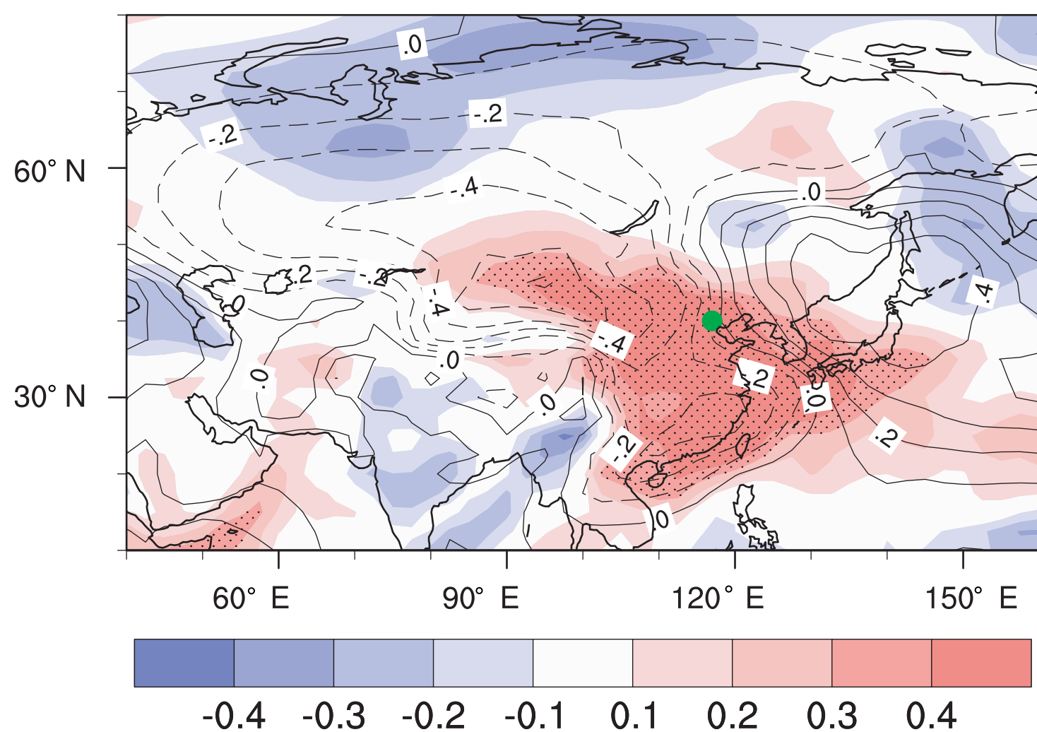
(a) Sea level pressure and near-surface specific humidity
