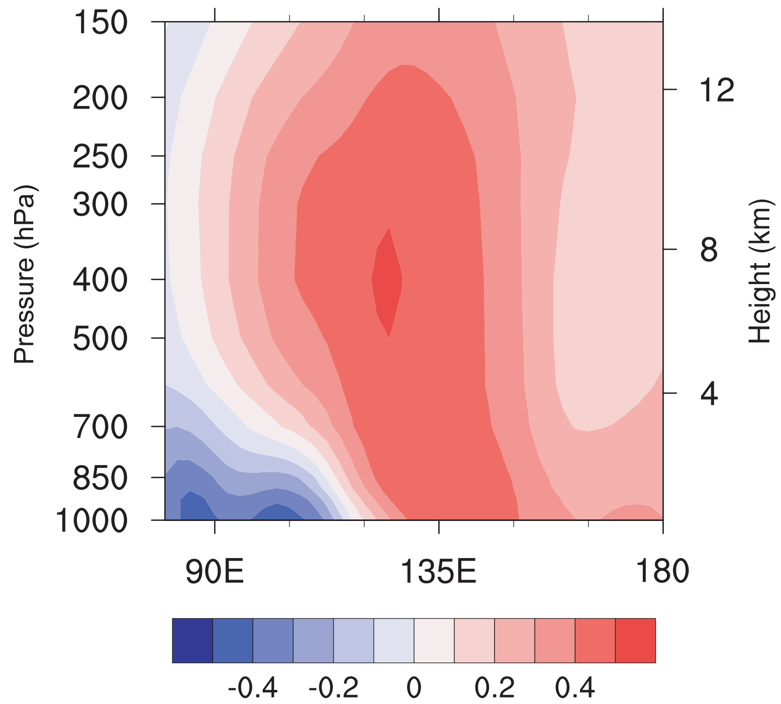
(f) Geopotential height
