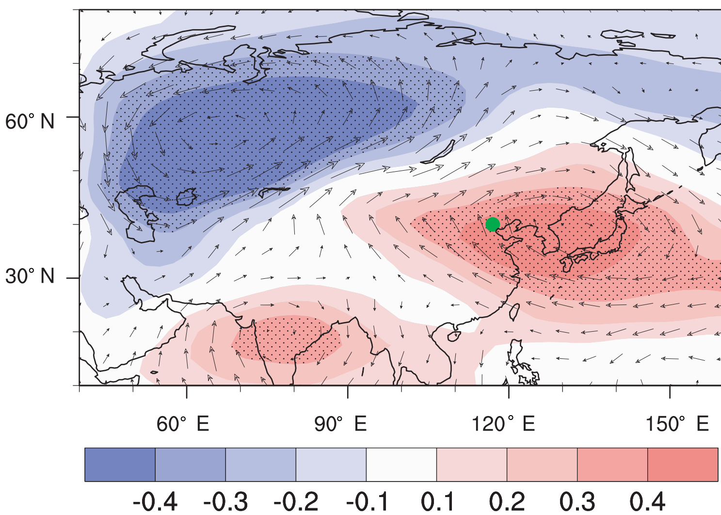
(c) Geopotential height and wind at 500 hPa
