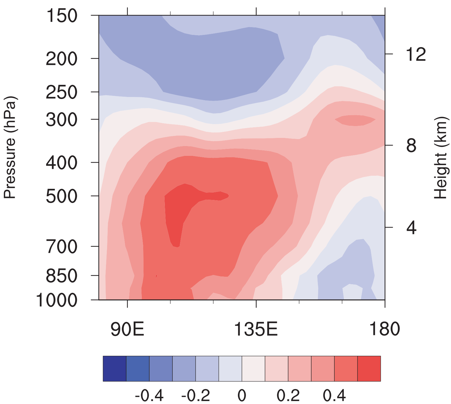
(e) Air temperature
