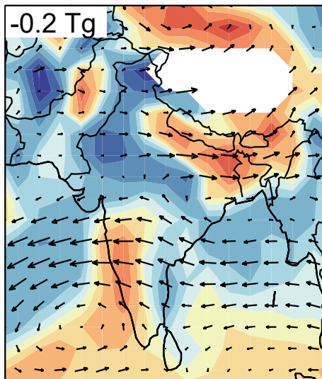
(e) \text{O}_3 horizontal transport [ 10^{-3} \text{ kg m}^{-2} ]
