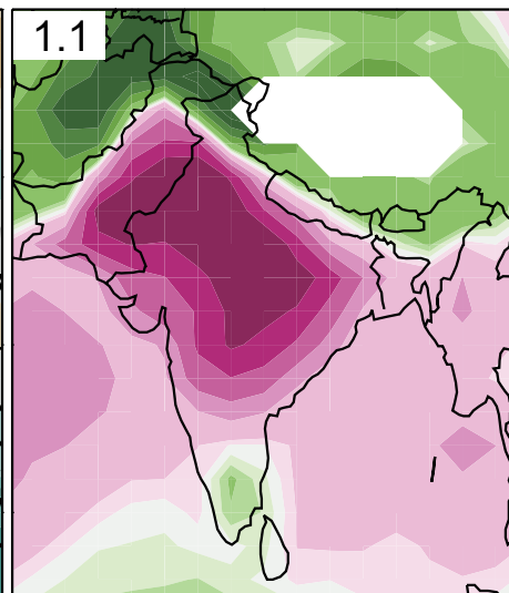
(c) Surface temperature [ ^{\circ}\text{C} ]
