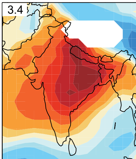
(a) Ozone [ppbv]
