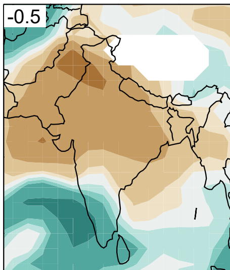
(b) Specific humidity [ \text{g kg}^{-1} ]
