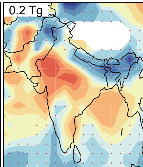
(f) \text{O}_3 vertical transport [ 10^{-3} \text{ kg m}^{-2} ]
