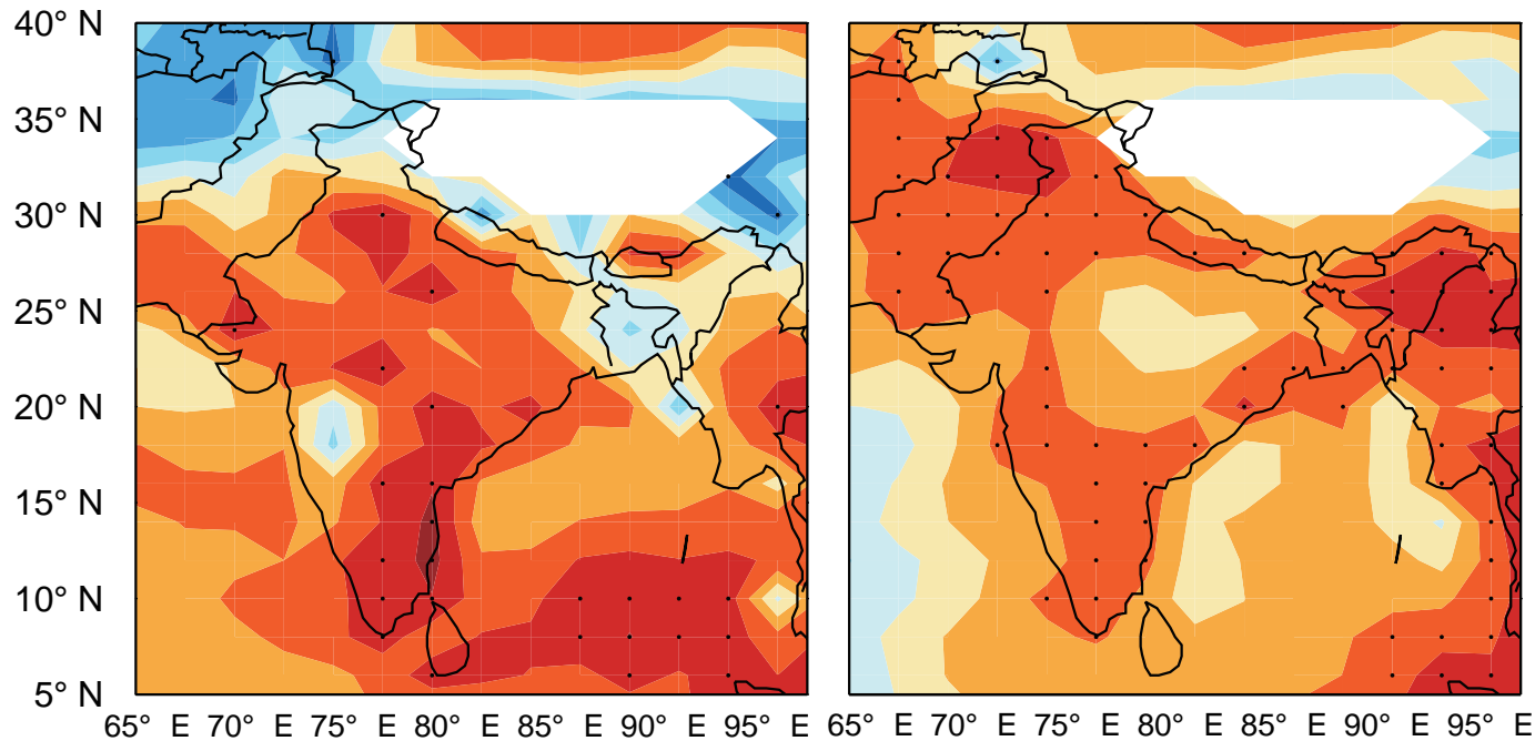
(a) OMI (2006–2014)
