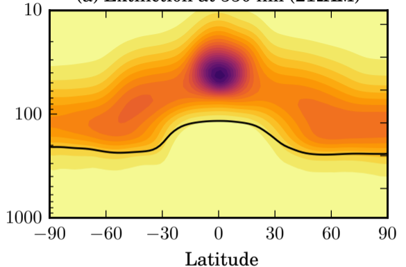
(a) Extinction at 550 nm (21_KM)
