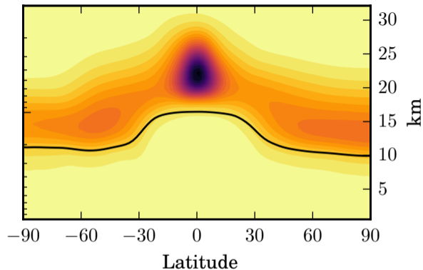
(b) Extinction at 550 nm (NORAD)
