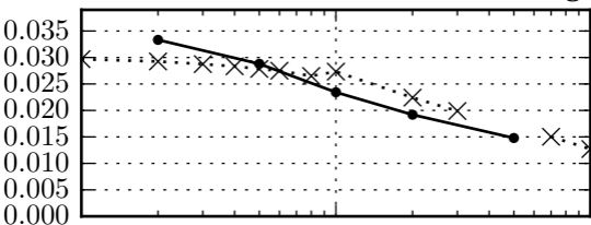
(c) AOD/burden [ \text{unit AOD}(550 \text{ nm}) / \text{Tg(S)} ]
