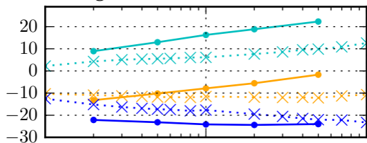
(b) Forcing/AOD [ \text{W m}^{-2} / \text{unit AOD}(550 \text{ nm}) ]
