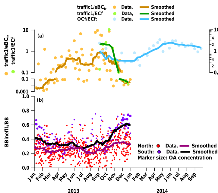
Figure 11. (a) Time series of traffic1 normalized to eBC tr and EC f in comparison to OC f /EC f in Magadino and (b) influence of inefficient wood burning emissions (BBineff1) in comparison to the sum of wood-burning-influenced factors (BB = BBineff1 + BBineff2 + BBeff) for the entire dataset.
