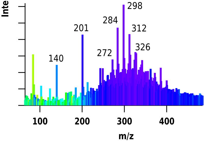
(c) San Vittore, 2013-12-14, R_{m/z,levoglucosan}
