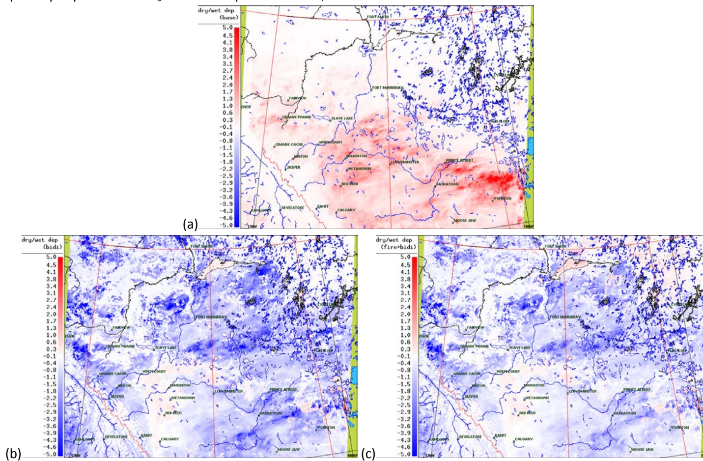
Figure A: Map of dry deposition of \text{NH}_3 over wet deposition of \text{NH}_4^+ ratios.
