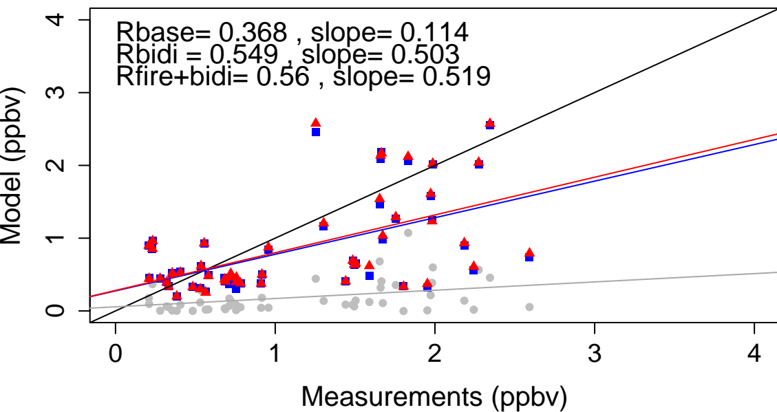
(c) Hourly average NH 3 concentrations on all flight paths
