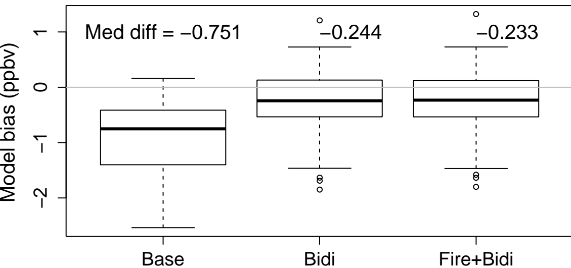
(c) Hourly average NH 3 concentrations on all flight paths
