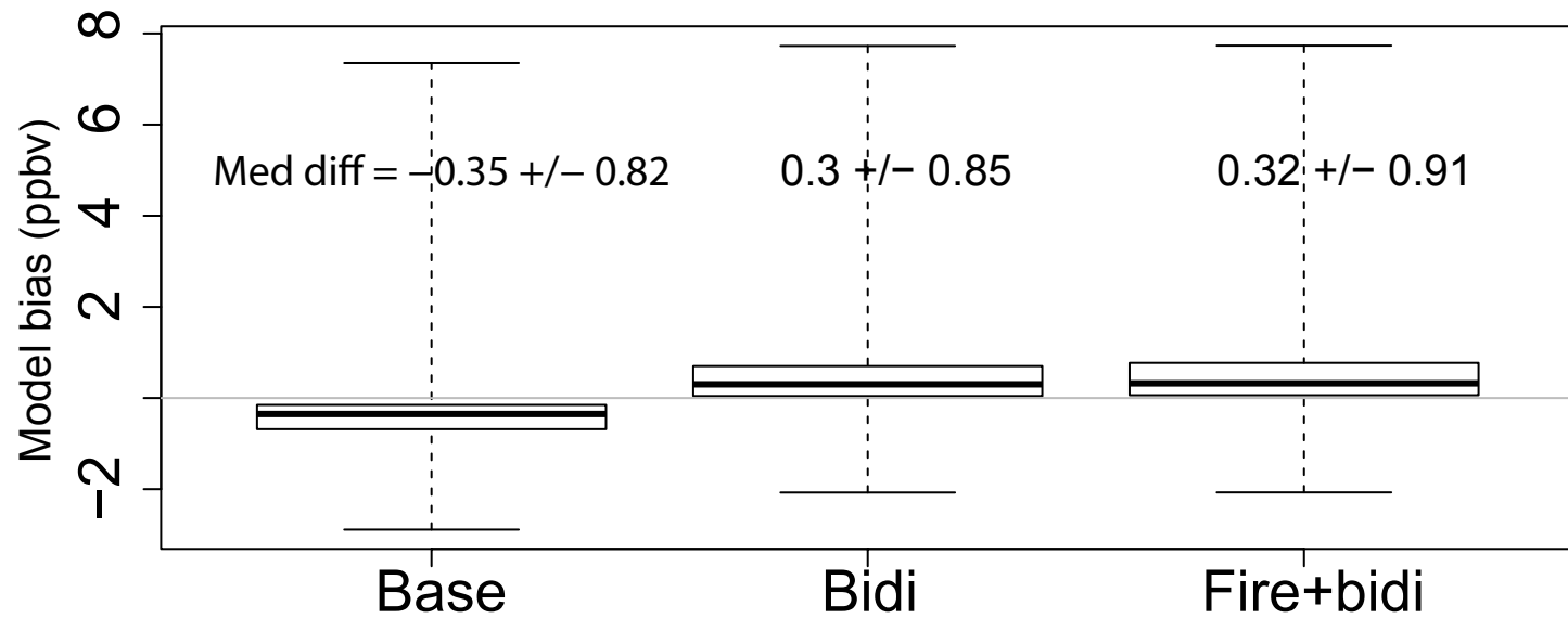
(a) NH 3 model bias at AMS13 site
