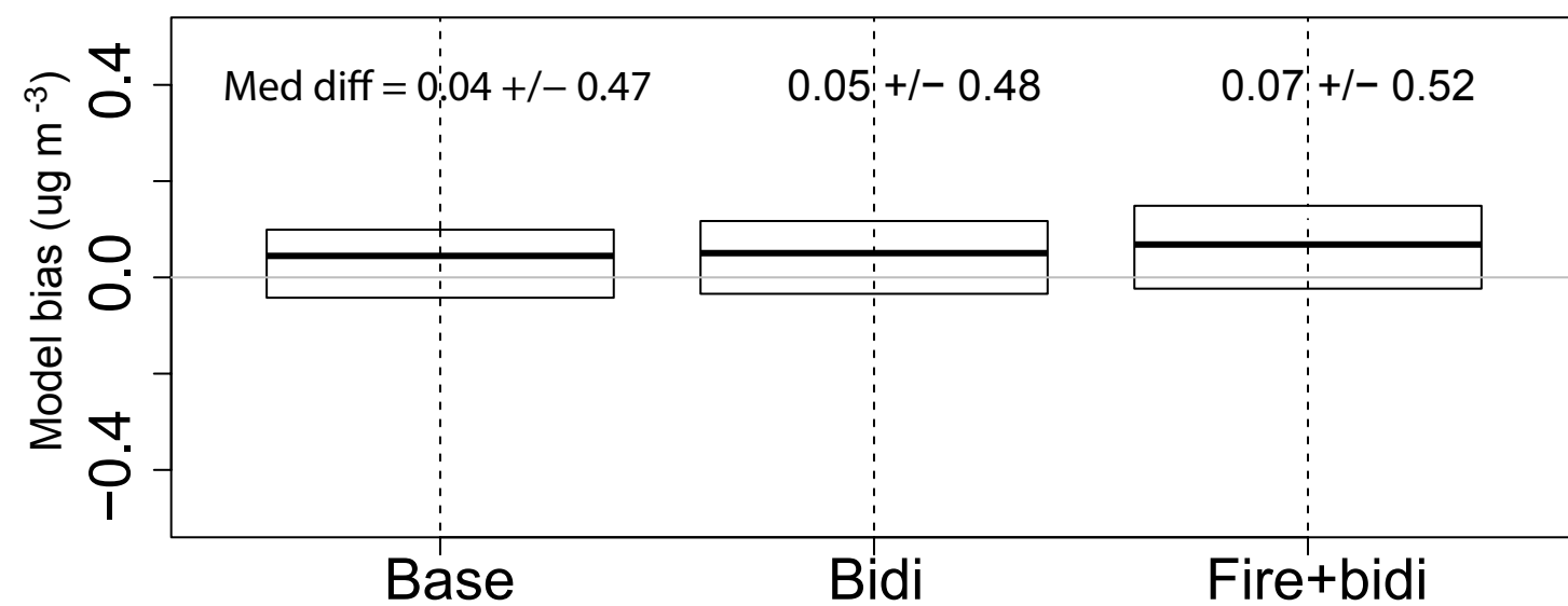
(b) Fine-mode NH 4 model bias
