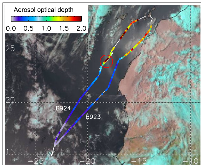
Figure 3. Meteosat Second Generation “321 RGB” image for 12 August at 16:30 UTC, showing the extent of the dust plume advected off the west coast of Africa. The track of flights B923 and B924 is overlaid. A colour scale depicts the lidar-derived AOD, and a red circle indicates the location where the aircraft descended to sample the heavy dust in situ. A SLR at 30 m altitude was performed between 15:52 and 16:04 UTC (run 4), and a SLR at 1000 m took place between 16:09 and 16:29 UTC (run 5).
