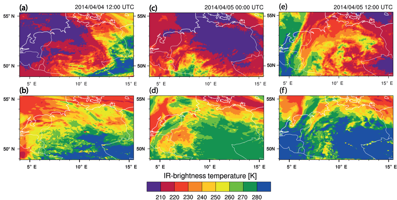
Figure 7. Infrared (IR; 8.7 \mu\text{m} channel) brightness temperature maps based on (a, c, e) MSG SEVIRI data of EUMETSAT (a, c, e) and (b, d, f) on the infrared simulation with the model output fields of the run SMLBK.
