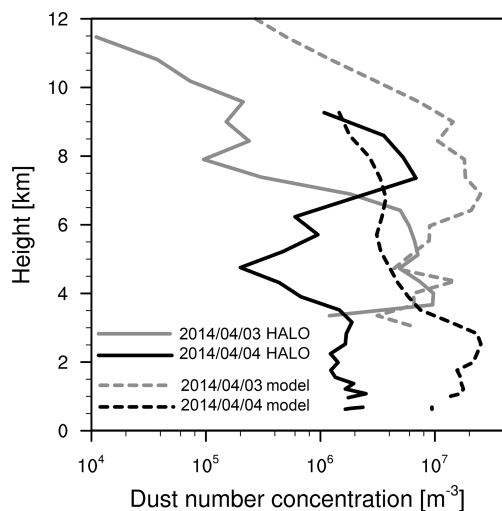
Figure 5. Vertical profiles of particle number concentration ( d > 500\text{ nm} ) as a proxy for dust) retrieved from aircraft measurements using an OPC and extracted model data along the flight paths shown in Fig. 14. Grey lines show data from 3 April 2014, black lines from 4 April 2014.
