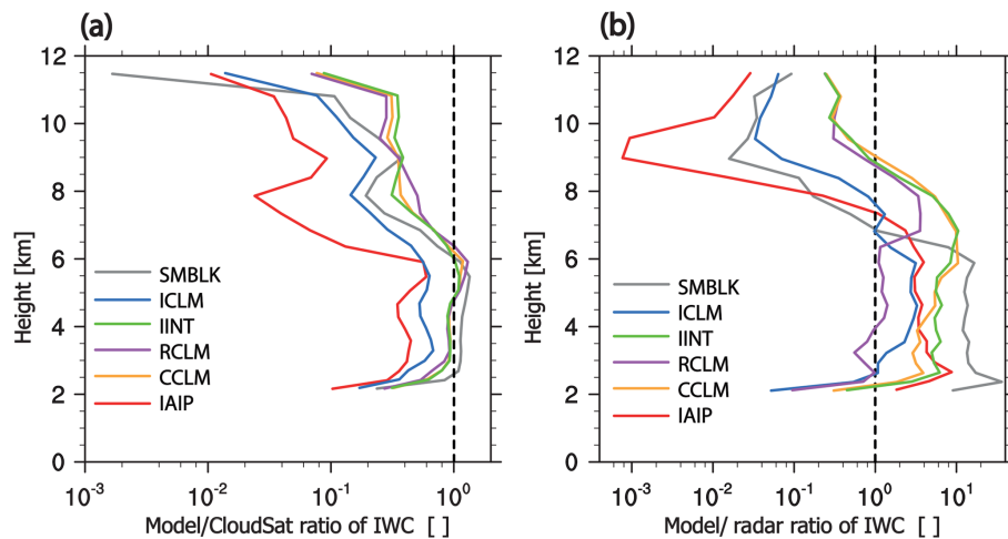
Figure 13. Vertical profiles of model–measurement ratios of IWC for (a) the CloudSat overpass on 4 April at 12:00 UTC and (b) for the time averaged radar observations at TROPOS site in Leipzig (51.3° N, 12.3° E).
