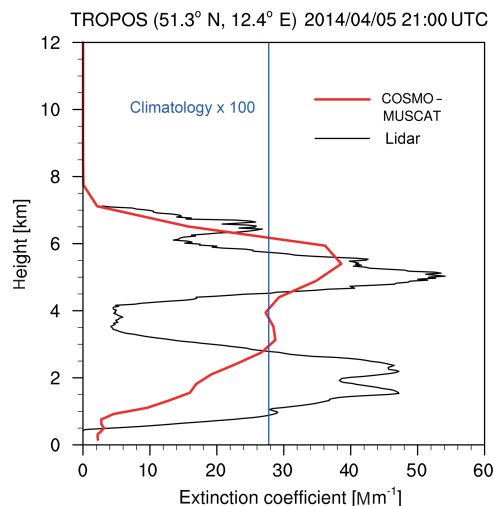
Figure 6. Vertical profile of aerosol extinction coefficient retrieved from lidar observations obtained at TROPOS in Leipzig on 5 April at 21:00 UTC, and calculated from the modeled dust fields at the nearest grid point.
