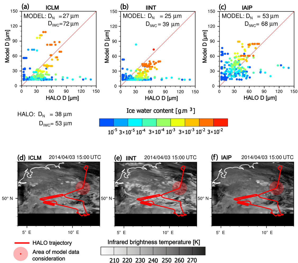
Figure 16. (a, b, c) Scatter plots of ice particle diameter D_i measured aboard HALO during ML-CIRRUS against model results for the model runs ICLM, IINT and IAIP, respectively. \bar{D}_N is the number-weighted average of D_i , \bar{D}_{IWC} is the IWC-weighted average of D_i . (d, e, f) Simulated infrared images for model runs ICLM, IINT and IAIP overlaid with HALO flight track and a reddish shaded circle, within which model data are considered for the comparison.
