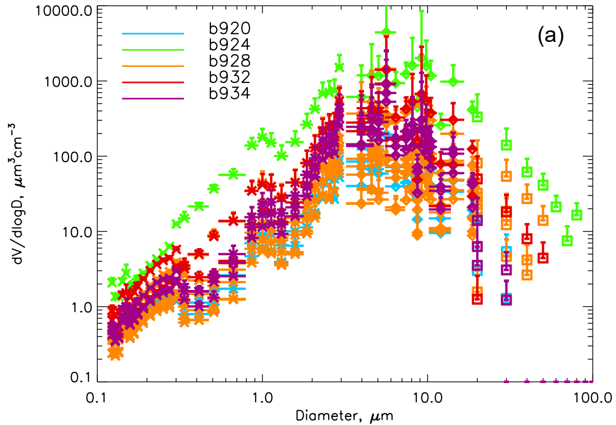
AER-D SAL size distribution, 2DS XY
