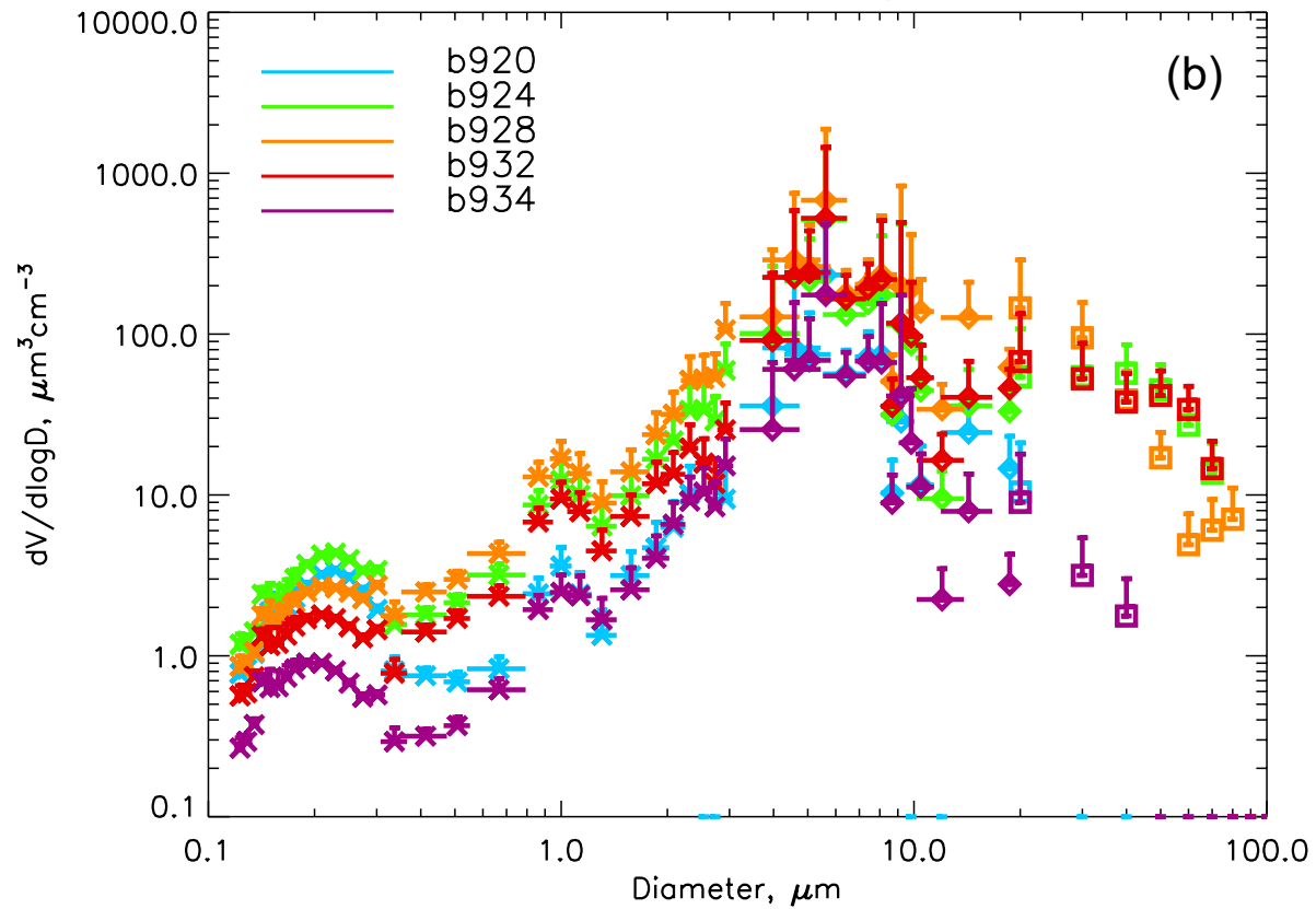
AER-D MBL size distribution, 2DS XY
